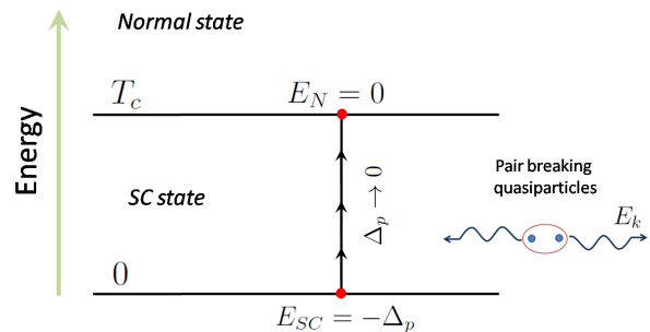
FIG. 1. (Color online) Excitation process in a conventional superconductor described by BCS theory [2]. Breaking a Cooper pair gives rise to two quasiparticles with energy E_k . The excitation is of fermionic type. As the temperature increases, more and more quasiparticles are created (pair breaking) leading to the decreasing of the gap \Delta_p(T) . The normal state is recovered at the critical temperature T_c , where \Delta_p(T_c) = 0 .
