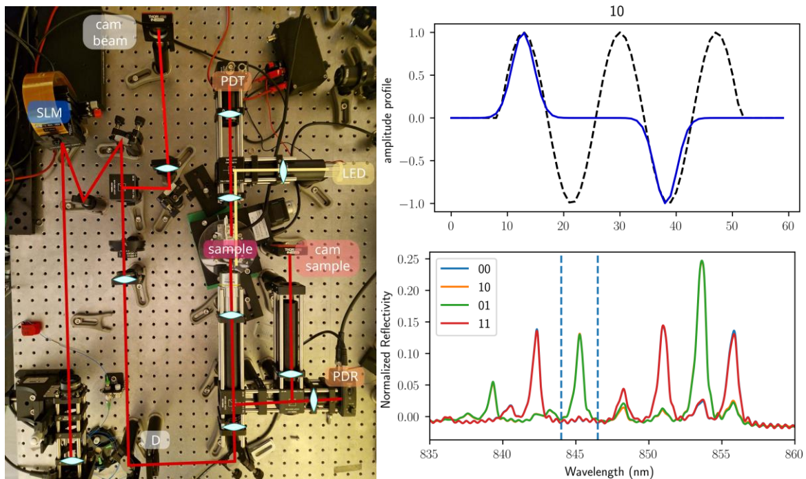
Figure 1. left : optical setup used. Top right: pentalobe mode shape (black dashed line) and mode superposition used in a typical combination experiment (blue line). Here the symbol 0 (nul phase) and 1 ( \pi phase) is shown. Bottom right: reflectivity spectra recorded for different phases. The dashed blue lines highlight the pentalobe mode resonance peak.
