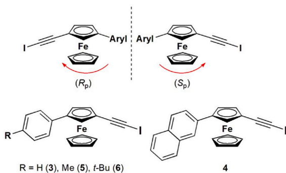
Fig. 3. Structures of planar chiral 1-(iodoethynyl)-3-arylferrocenes 3–6 . ( R_p )- and ( S_p )-enantiomers are also depicted.
