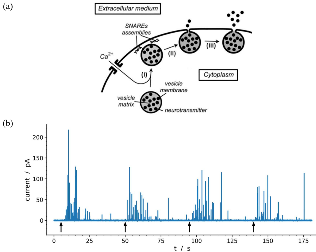
Fig. 1. a) Schematic representation of the main exocytotic release steps 10 : (I) Ca 2+ -driven docking of a primed exocytotic vesicle; (II) opening of the fusion pore and beginning of release; (III) final opening of fusion pore and main releasing phase (for simplicity the SNAREs assemblies are only represented at the end of phase I because they play a crucial role in the docking mechanism; 18,19 for the same reason the membrane cytoskeleton, see Fig.3 in previous work 9 , is not shown). b) Representative amperometric data from a single PC12 cell with highly loaded vesicles 12 recorded in HEPES buffer with 5 \mu\text{m} carbon fiber electrode held at +680 mV vs Ag/AgCl. The 4 distinct groups of spikes seen in the trace were elicited by a series of 5 s duration 105 mM K + puffs (each arrow indicates the beginning of K + pulse for each group). Most of the events displayed in the trace (84%) were analyzable through the model developed here including 97 spikes exhibiting two-exponential tails and 9 single-exponential ones (see Table 1 and Fig 7).
