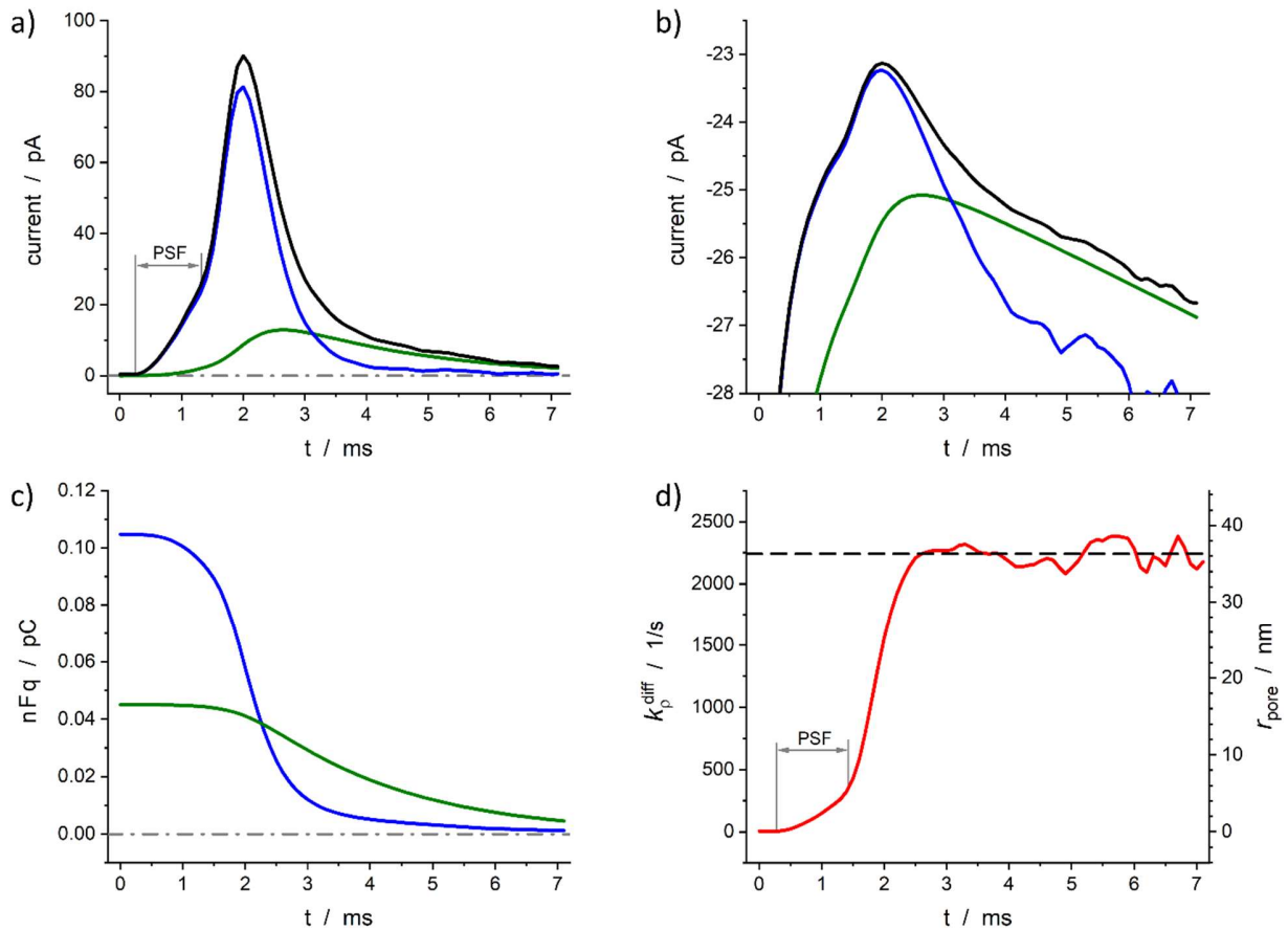
Fig.6. Quantitative analysis of a typical amperometric spike featuring dopamine release monitored at a PC12 cell with CFE. Current spike and its reconstructed compartment-wise components in linear (a) and semi-log (b) scales. Variation of NT content in each domain (c) and reconstructed opening dynamics (d). The dashed line in (d) represents k_{max}^{diff} ; the right vertical axis indicates the corresponding r_{pore} values which were evaluated assuming D_{ves}/r_{ves}^2 = 5803 \text{ s}^{-1} 33 and r_{ves} = 94 \text{ nm} . 33 PSF in (a) and (d) stands for “pre-spike feature”.
