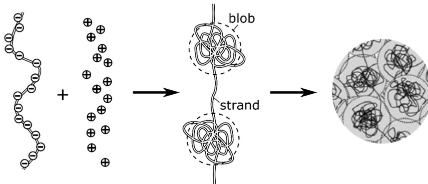
Fig.3. Schematic representation of the intravesicular structure of the secretory vesicle (the terminology “blob” vs. “strand” was introduced by de Gennes).
