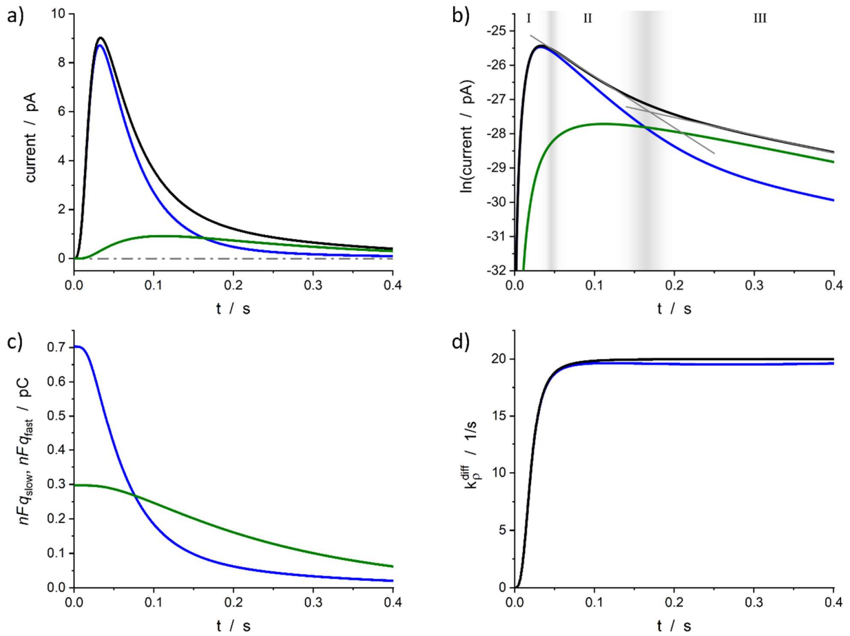
Fig.4. Simulated spike and its reconstructed components in real (a) and semi-log (b) scales. (c)
