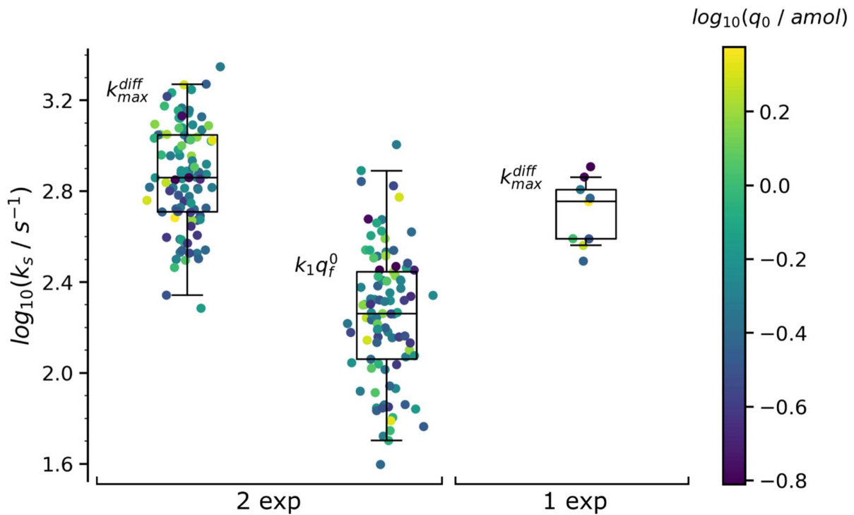
Fig. 7. Box and whisker plots of the reconstructed k_{max}^{diff} and k_1 q_f^0 values for the 97 spikes with two exponential decay and k_{max}^{diff} for the 9 spikes with single exponential decay (spikes from the trace in Fig.1b). The color of each dot refers to the reconstructed releasable content of a vesicle q_0 (in amol) as indicated by the color bar on the side. The different horizontal segments in each box and whisker plot represent, from top to bottom, the upper extreme (90%), upper quartile (75%), median (50%), lower quartile (25%) and lower extreme (10%) probabilities.
