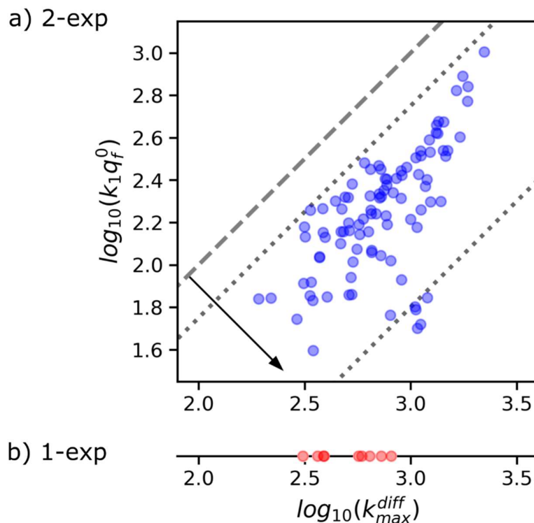
Fig.8. (a) Correlation between k_{max}^{diff} and k_1q_f^0 values characterizing each of the 97 spikes exhibiting two-exponential tails analyzed from the amperometric trace in Fig. 1b. These are put in perspective with the k_{max}^{diff} values (b) determined for the 9 spikes displaying a single-exponential tail recorded in the same amperometric trace. Slanted dotted lines delimit the region in which the spikes with two exponential tails may be quantitatively analyzed owing to the experimental constraints (see text and Fig 9).
