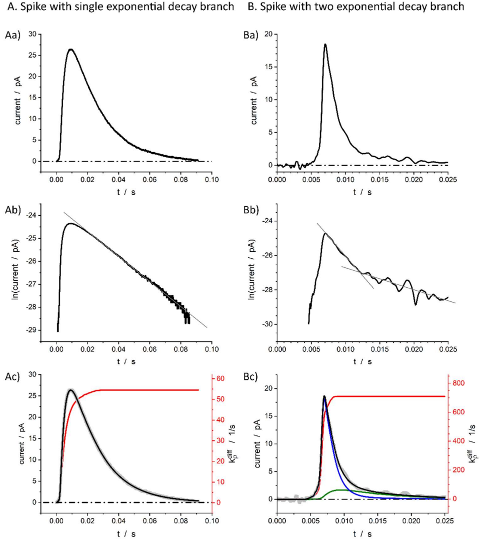
Fig.2. Single (A) and double exponential (B) spikes in linear (a) and semi-log (b) scales; c) shows simulation results of the spike current (black), its components (blue and green in Bc, see below for the meaning) and fusion pore opening dynamics (red, see text for k_p^{diff}(t) definition) with k_{\rho_{max}}^{diff} = 54.5 \text{ s}^{-1} in (Ac) and k_{\rho_{max}}^{diff} = 710.0 \text{ s}^{-1} in (Bc). The grey symbols are the overlaid experimental spikes shown in (a). The spike (A) was obtained from a chromaffin cell, while spike (B) is from a PC12 cell. Assuming D_{ves}/r_{ves}^2 = 415 \text{ s}^{-1} , 27 r_{ves} = 156 \text{ nm} 32 for chromaffin cells and D_{ves}/r_{ves}^2 = 5.8 \times 10^3 \text{ s}^{-1} , 33 r_{ves} = 95 \text{ nm} 33 for PC12 cells, the maximum pore opening can be evaluated as r_{pore}^{max} = 20 \text{ nm} and r_{pore}^{max} = 12 \text{ nm} , respectively.
