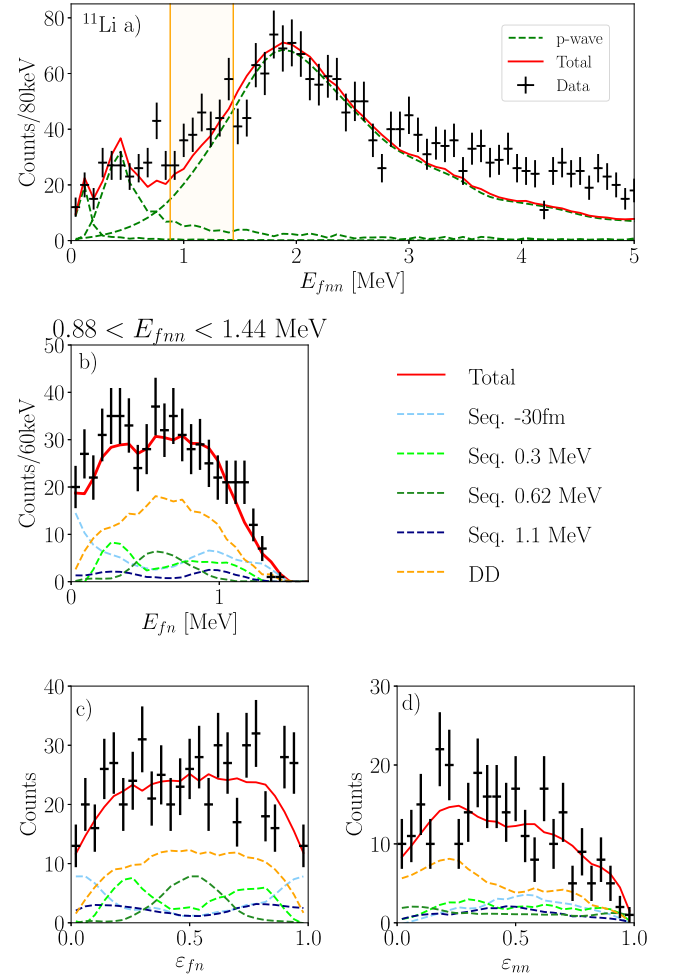
Fig. 2. Fits of the 3B, 2B and reduced energy spectra of ^{11}\text{Li} . “Seq. -30 fm”, “Seq. 0.3 MeV”, “Seq. 0.62 MeV” and “Seq. 1.1 MeV” relate to the sequential decay, via the virtual state with a_s = -30 fm, the 0.3 MeV resonance, the 0.62 MeV resonance and the 1.1 MeV resonance, respectively, in ^{10}\text{Li} . “DD” relates to the direct decay of the 2.13 MeV resonance in ^{11}\text{Li} . a) ^{11}\text{Li} 3B relative energy spectrum; b) ^{10}\text{Li} 2B relative energy spectrum gated on 0.88 < E_{fnn} < 1.44 MeV; c) ^9\text{Li} 2B reduced relative energy spectrum for the same gate as b); d) 2B n+n reduced relative energy spectrum for the same gate as b). The slice of 3B relative energy spectrum presented here is shaded in panel a).
