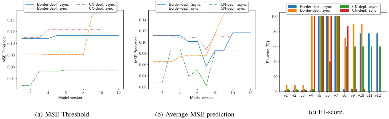
(a) MSE Threshold. (b) Average MSE prediction (c) F1-score. Fig. 9: Quality of the generated model version for anomaly detection as the learning process evolves
