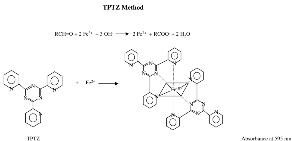
Fig. 2. Schematic reactions for the PSA, MBTH, and TPTZ methods. Note that the unreacted reagents \text{KBH}_4 and \text{HIO}_4 for the MBTH are quenched using \text{HCl} and \text{NaAsO}_2 , respectively.
