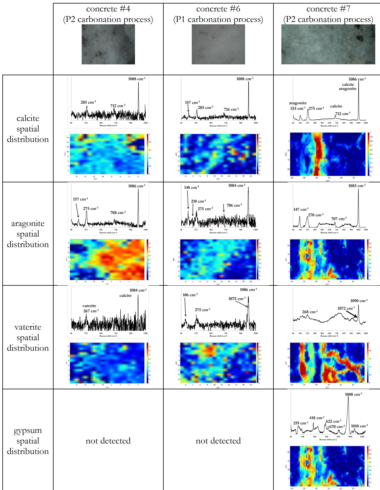
Figure 7: 2D-spatial normalized distribution of CaCO 3 polymorphs, as obtained by MCR-ALS (non-negativity and unimodality constraints, 40-1200 cm -1 spectral range) performed after a SIMPLISMA initialization on PP1-corrected Raman maps containing both the old and the new cement pastes.
