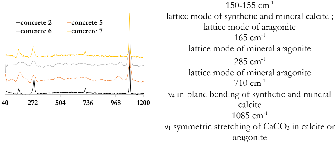
Figure 3: Selected normalized Raman spectra obtained on polished surfaces of RCA-containing concretes 2, 5, 6 and 7 ( \lambda_{\text{laser}} = 514 \text{ nm} , x50 magnification. The spectra were offset for clarity).
