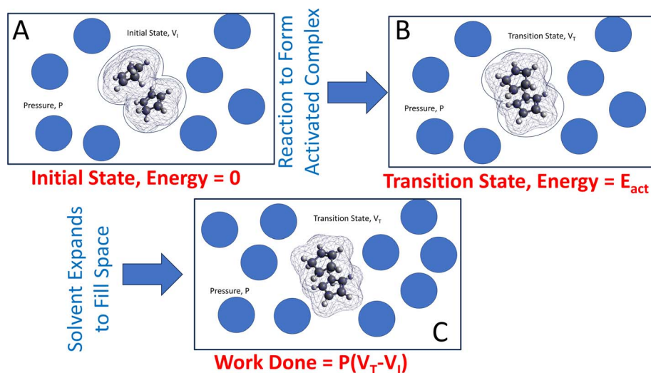
Fig. 1 Illustration of a calculation of the Gibbs free energy due to a hydrostatic pressure P for the Diels–Alder cycloaddition dicyclopentadiene showing (A) the initial-state structure shows the atom positions enclosed in a van der Waals' cage. (B) The transition-state structure with an energy E_{act} , which has a smaller volume than the initial-state structure. (C) The space created by the transformation is filled by the surrounding solvent where the contribution to the Gibbs free energy is P(V_T - V_I) .
