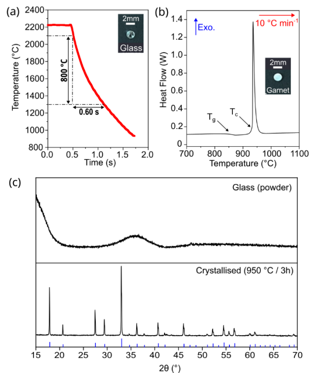
Figure 2. Synthesis of \text{Gd}_{3.2}\text{Al}_{4.8}\text{O}_{12} by glass crystallization. (a) Temperature profile of a \text{Gd}_{3.2}\text{Al}_{4.8}\text{O}_{12} melt free-cooled in an oxygen jet, resulting in a glass bead (see photograph, inset). (b) DSC scan recorded on \text{Gd}_{3.2}\text{Al}_{4.8}\text{O}_{12} glass powder (crushed beads) on heating at 10\text{ }^\circ\text{C min}^{-1} , showing a glass transition ( T_g ) at \sim 850\text{ }^\circ\text{C} and the onset of crystallization ( T_c ) at \sim 925\text{ }^\circ\text{C} . Inset, photograph of a crystallized \text{Gd}_{3.2}\text{Al}_{4.8}\text{O}_{12} bead. (c) Laboratory PXRD scans of glass powder before (upper panel) and after (lower panel) thermal treatment at 950\text{ }^\circ\text{C} for 3 hours, with the crystalline phase indexed to a cubic garnet structure (blue stick diagram, base of frame).
