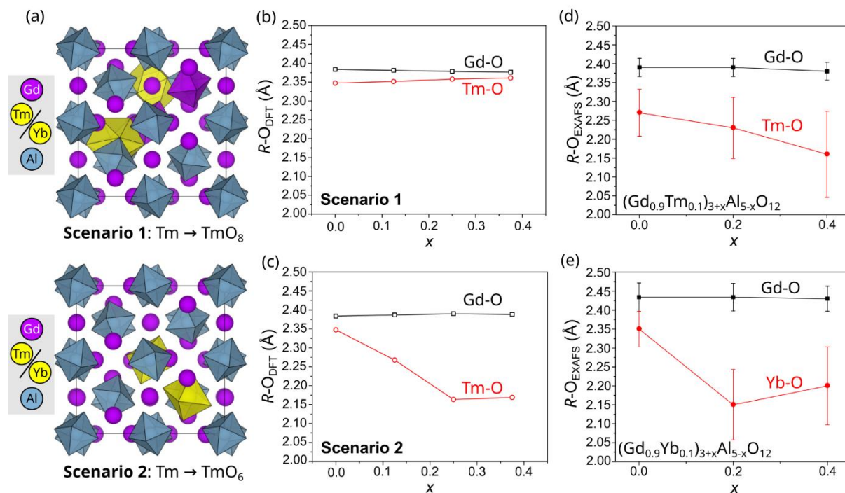
Figure 5. Site preferences of \text{Tm}^{3+} and \text{Yb}^{3+} dopants by EXAFS and DFT (a) Two representative unit cells relaxed by DFT, from Scenario 1 ( \text{Tm}/\text{Yb}^{3+} populates A sites) and Scenario 2 ( \text{Tm}/\text{Yb}^{3+} populates B sites) respectively, both with x = 0.25 . The C sites are omitted for clarity. (b, c) DFT-calculated trends in Gd-O and Tm-O distances, according to Scenario 1 and Scenario 2. (d, e) Experimental trends in R -O distances ( R = \text{Gd}, \text{Tm} or \text{Yb} ) derived from EXAFS spectra, exhibiting Scenario 2-like behavior.
