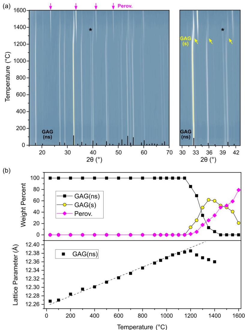
Figure 4. In-situ PXRD of \text{Gd}_{3.4}\text{Al}_{4.6}\text{O}_{12} collected on heating from room temperature to 1600^\circ\text{C} . (a) Two dimensional plot of the region 15 \leq 2\theta \leq 70^\circ . Expected peaks/intensities from \text{Gd}_{3.4}\text{Al}_{4.6}\text{O}_{12} “GAG(ns)” are shown by the black stick diagram at the base of the frame. Peaks due to \text{GdAlO}_3 “Perov.” are indicated by magenta arrows at the top of the frame. The peaks corresponding to stoichiometric \text{Gd}_3\text{Al}_5\text{O}_{12} “GAG(s)” are indicated by yellow arrows in the zoomed panel. Peaks from the platinum sample holder are marked by asterisks. (b) Rietveld-refined weight percentages of \text{Gd}_{3.4}\text{Al}_{4.6}\text{O}_{12} , \text{Gd}_3\text{Al}_5\text{O}_{12} and \text{GdAlO}_3 as a function of temperature (top panel) and the lattice parameter evolution of \text{Gd}_{3.4}\text{Al}_{4.6}\text{O}_{12} (bottom panel) showing abrupt changes at \sim 1200^\circ\text{C} . The dashed line is a guide to the eye.
