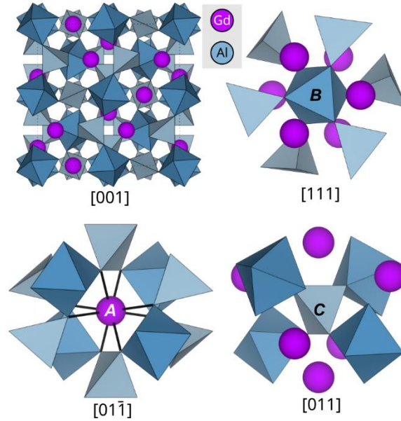
Figure 1. Unit cell of the cubic garnet structure of Gd_3Al_5O_{12} projected along [001] (cell edges marked by dashed line), with structural fragments showing the local A, B and C cation environments.
