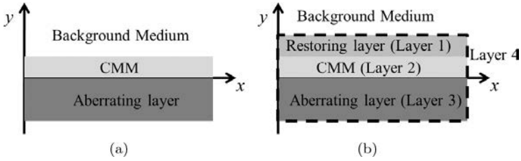
Fig. 2.21. (a) Schematic of the CMM, the aberrating layer, and the background medium. (b) Schematic of acoustic cloaking using CMM, the dashed lines indicate the boundaries of layer 4.
