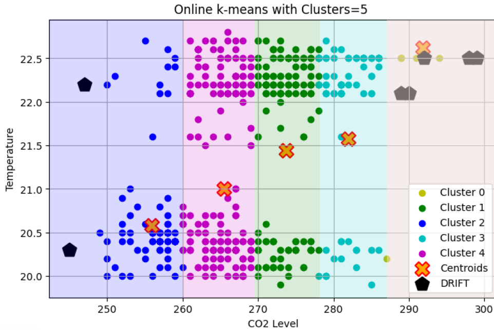
Figure 5: Applying KMeans Clustering with Micropython-ulab and K=5
