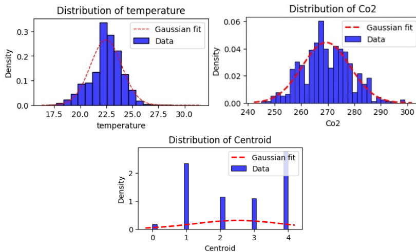
Figure 4: Distribution of Data
