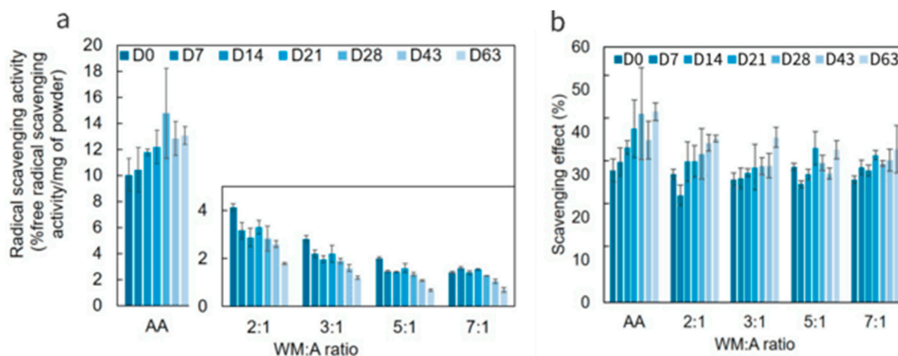
Figure 6. Radical scavenging activity of MDGA-AA particles according to the wall materials/active (WM:A) ratio (a) and at 0.3 g/L of ascorbic acid (AA) equivalent (b). Error bars represent the standard deviation values.
