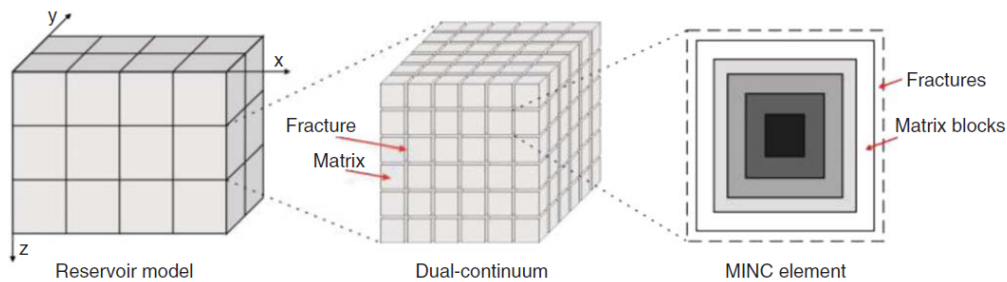
Figure 11: Concept of the multiple interacting continua (MINC) method ((Jiang et al., 2016) redesigned form of original (Pruess and Narasimhan, 1982).
