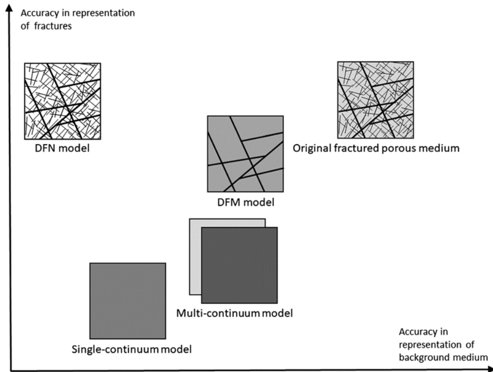
Figure 3: Conceptual approach for fractured porous media (Berre et al., 2019b)
