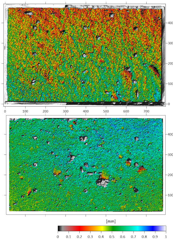
Figure 15: Colored fracture aperture distribution at artificial granite block fracture
