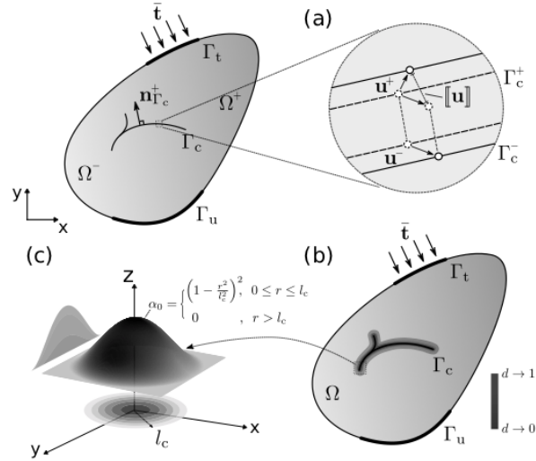
Figure 5: Graphical comparison of numerical methods for description of discontinuities (Yoshioka et al., 2019)
