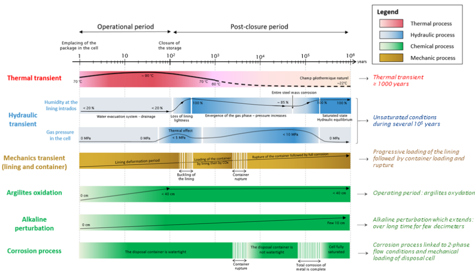
Figure 1: Thermal, hydraulic, mechanical, chemical processes concomitance affecting repository and geological environment during operational and post-closure period.
