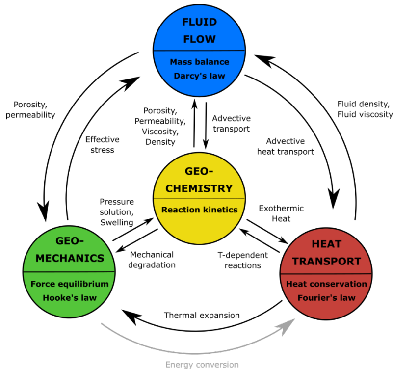
Figure 14: Schematic illustration of the coupled thermal-hydro-mechanical-chemical processes relevant to safety assessment of nuclear waste repositories (modified from Gaucher et al. (2015))
