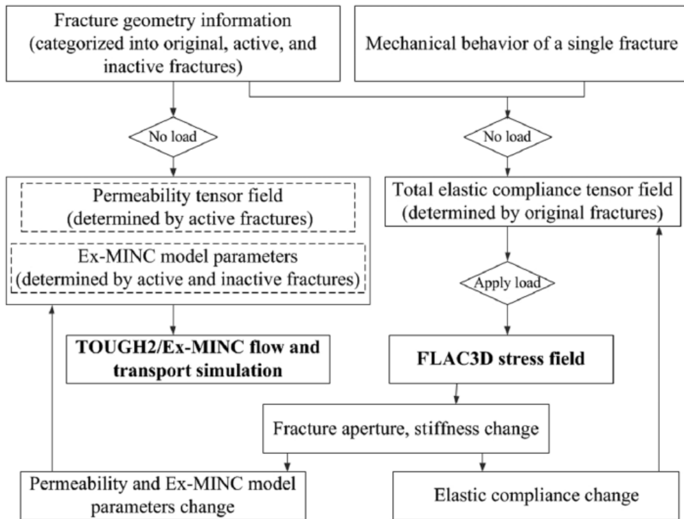
Figure 7: Scheme of the extended multiple interacting continua (Ex-MINC) method (Wang et al., 2014).
