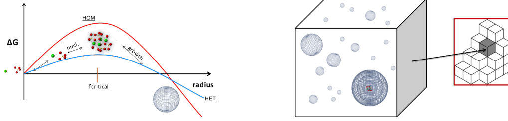
Figure 10: Cross scale precipitation modelling. (left) Classical nucleation Theory and energetic barriers to produce the critical nuclei for homogeneous (HON) and heterogeneous (HET) nucleation mechanisms. The two dimensional 9-velocity lattice (D2Q9), (right) Sub-lattice model for homogeneous nucleation which allows to model the evolution of reactive surface areas.
