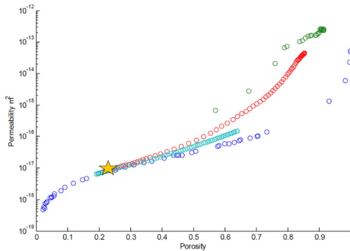
Figure 13: Evolution of permeability for different reactive transport dissolution scenario in a porous medium. Porosity permeability correlations can be extracted via fitting for use with macroscopic codes. Blue points represent the random set of geometries permeabilities that can serve as starting points (star). A geometry with 20% porosity is selected. Temporal evolution of the structure for three different cases were Peclet and Damkohler number vary.
