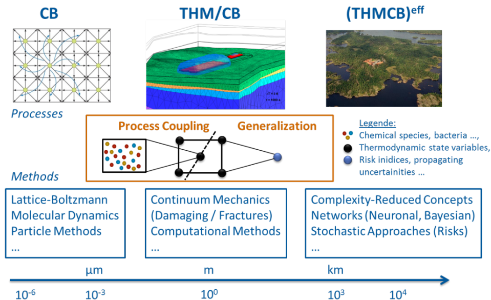
Figure 2: Vision for scale transition schemes: from process to management scales (figure sources: https://developer.nvidia.com , BGR (OGS simulation), Google Earth).
