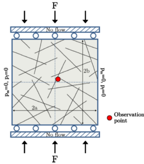
Figure 6: Problem used for benchmarking dual-continuum poroelastic models (Ashworth and Doster, 2019).
