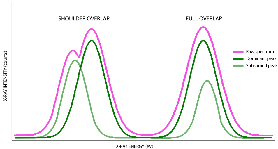
Figure 8. Schematic representation of the types of peak overlap that can occur in an XRF spectrum.
