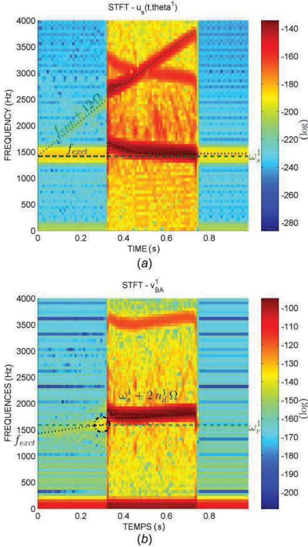
Fig. 10 STFT of the radial displacement of the casing and the tangential displacement of a blade tip with a fast speed ramp for \mu = 0.1 and k_w = 1 \times 10^{-12} \text{ Pa}^{-1} : (a) casing and (b) bladed disk
