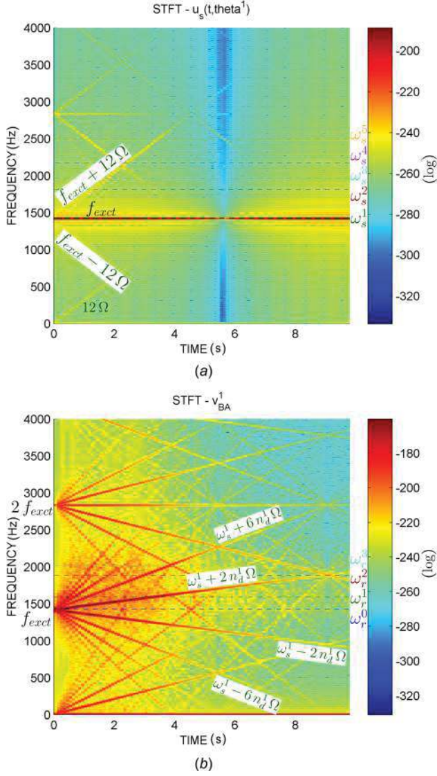
Fig. 14 STFT of the radial displacement of the casing and the tangential displacement of a blade tip with a slow speed ramp for \mu = 0.1 and k_w = 1 \times 10^{-12} \text{ Pa}^{-1} : (a) casing and (b) bladed disk
