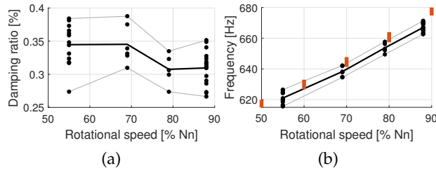
FIGURE 15. Evolution of the modal damping ratio (a) and the frequency (b) according to the rotational speed for the modal tests 2F-4ND. Red bars : FEM frequencies for N_v = 2 to 8.
