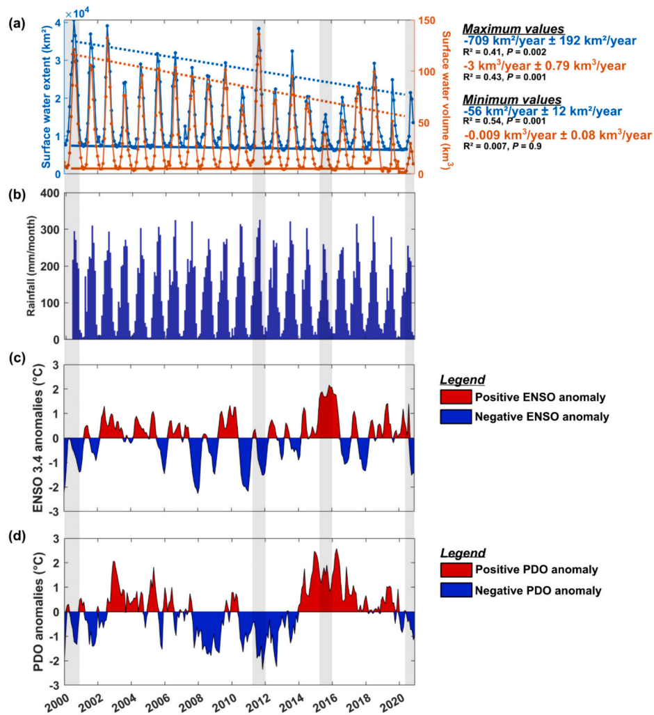
Fig. 3. Time series of the extent ( \text{km}^2 ) and volumes ( \text{km}^3 ) of surface water, rainfall ( \text{mm}/\text{month} ), and climatic indices ENSO and PDO anomalies ( ^{\circ}\text{C} ) over 2000–2020. a) Time series of surface water extent from multispectral imagery ( \text{km}^2 – blue) and surface water volumes ( \text{km}^3 – orange) over 2000–2020. For each time series, trend slopes of maximum values (dotted line) and minimum values (solid line) are displayed, -709 \pm 192 \text{ km}^2/\text{year} corresponds to a slope of -709 \text{ km}^2/\text{year} and a standard error of 192 \text{ km}^2/\text{year} with statistics ( R^2 is the coefficient of determination and P is the p -value), b) time series of rainfall data from GPM over 2000–2020, c) time series of anomalies of ENSO 3.4 and d) time series of PDO (Pacific Decadal Oscillation) indices anomalies over 2000–2020. Grey rectangles represent minimum and maximum values of inundation extent and surface water volumes, with rainfall, ENSO and PDO associated.
