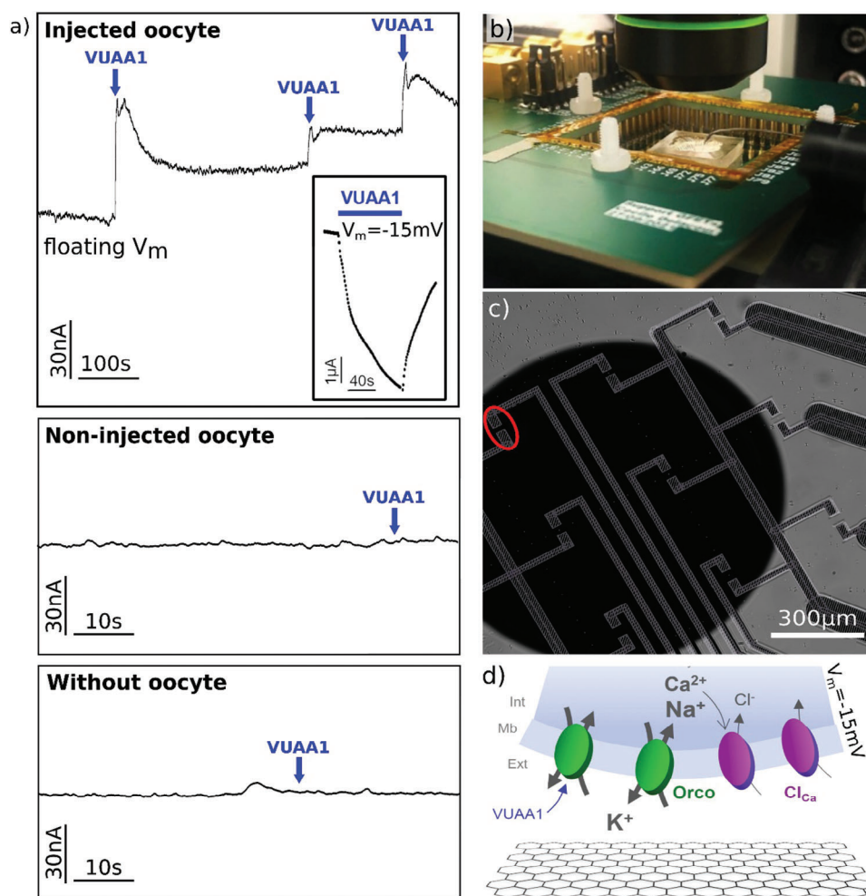
Figure 4. Real-time detection of Orco channel activation in Xenopus oocyte. (a) Timestamp of the drain current I_D during the three successive applications (30 \mu L) of Orco agonist VUAA1 (respectively 90, 183, and 260 \mu M). The same ligand application is repeated on non-injected oocytes (does not express the Orco protein) and G-FET without oocyte coupling. G-FET is polarized at V_{DS} = -20 mV. The acquisition frequency is 25 kHz. Inset: Typical response of TEVC to VUAA1 activation of Orco channels. By convention, the current is negative, and an increase in the current amplitude results in a downward deflection. (b) G-FET electronic set-up under transmission microscopy. The reference potential of buffer electrolyte (ND96) is fixed with a quasi-Pt reference electrode at V_g = 0 V. (c) The Xenopus oocyte is placed on a G-FET array using optical microscopy. G-FET used for Orco real-time measurements (a) is marked by a red circle. (d) Schematic showing the flow of ions through Orco (green) expressed in the plasma membrane of oocytes and when activated by VUAA1. Endogenous Cl_{Ca} channels are depicted in purple and activated by intracellular calcium. V_m is the transmembrane voltage of the Xenopus oocyte at the resting state.
