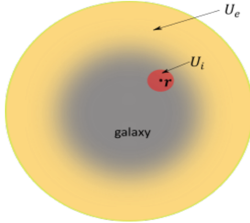
Fig 14 : Averaging over a ball surrounding a star or a galaxy
