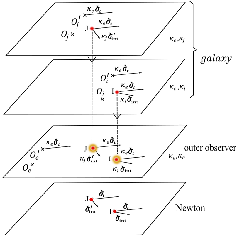
Fig 16 : Point of view of different observers
