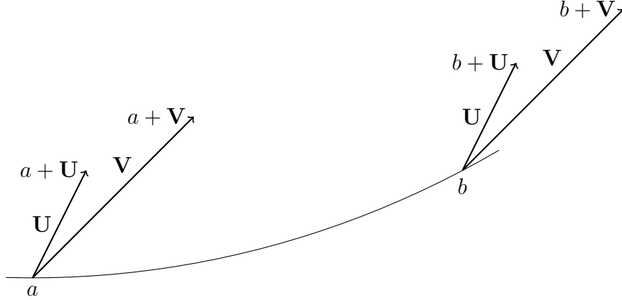
Fig 3 : Discrepancy in size measurement : d_a(a, a+U) = d_b(b, b+V) , while d_a(a, a+U) \neq d_a(b, b+V) .
