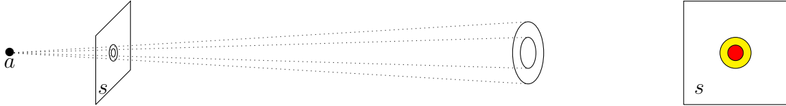
Fig 6.a : Images obtained without \kappa -effect, the annulus is represented in yellow,; the central disk is represented in red
