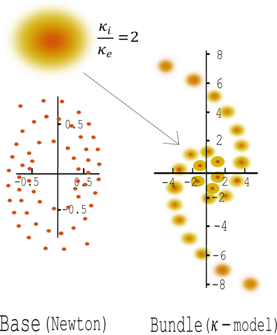
Fig 9 : A toy example : A well-developed conservative spiral substructure seen in the bundle as opposed to its counterpart living in the base (a tightly coiled spiral)
