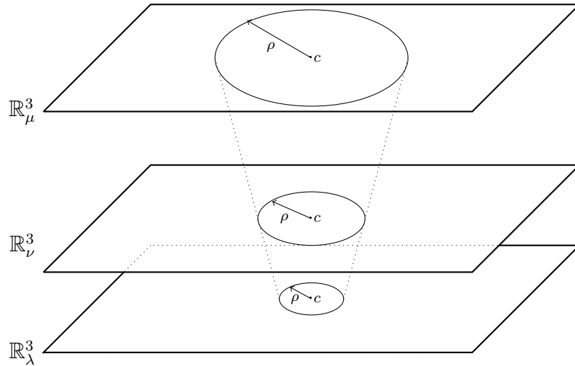
Fig 2 : Circles with same radii and centers
