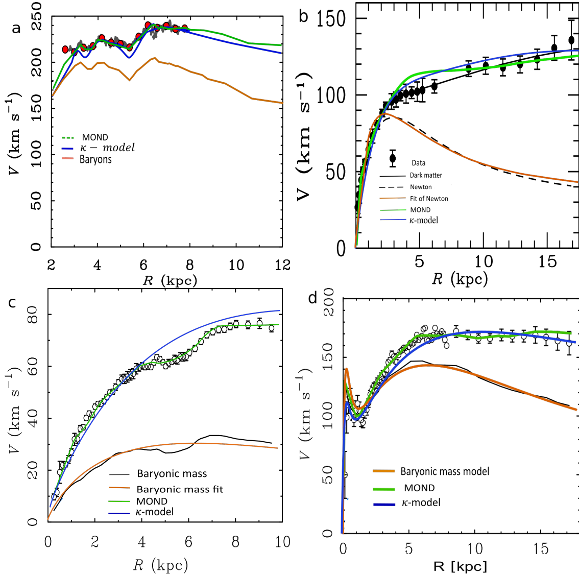
Fig 8 : Galaxy rotation velocity profiles: a. The Milky Way in the vicinity of the Sun, b. M33, c. NGC 1560, d. NGC6946. For the details see [2].
