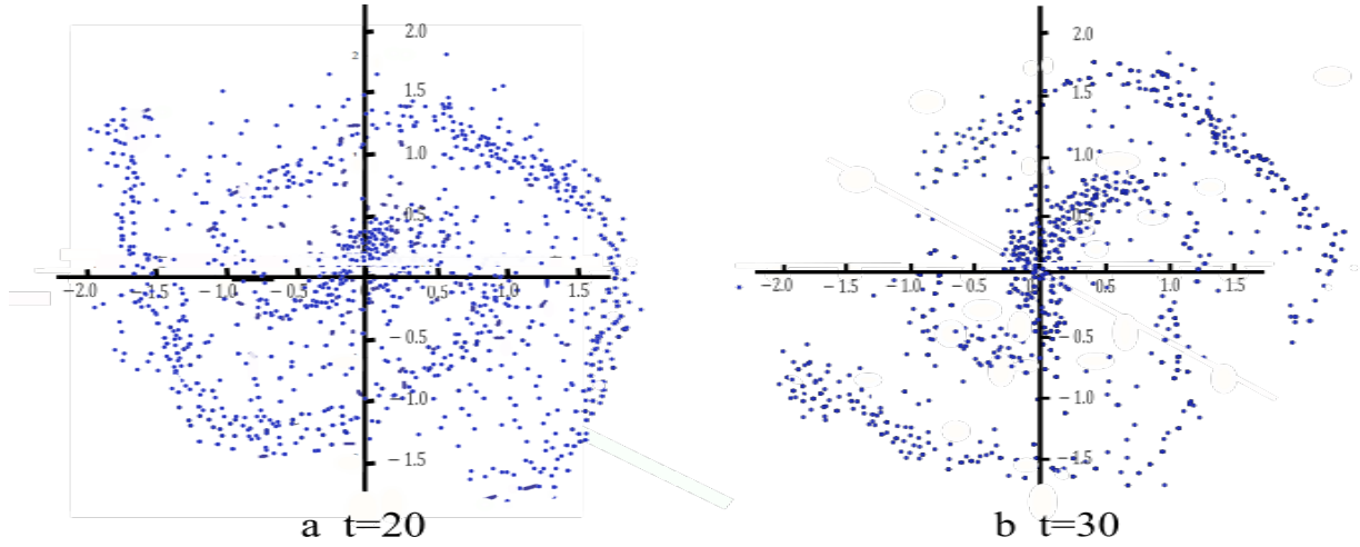
Fig 10 : A conservative grand design spiral produced by a numerical simulation in the \kappa -model framework (for the details see [2]). The elapsed time is given in the unit of 100 Myr. The Newtonian equivalent would be a much tighter spiral with a larger number of turns.
