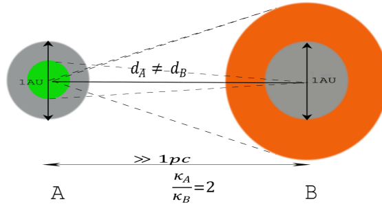
Fig 4 : Discrepancy in size measurement for a disk
