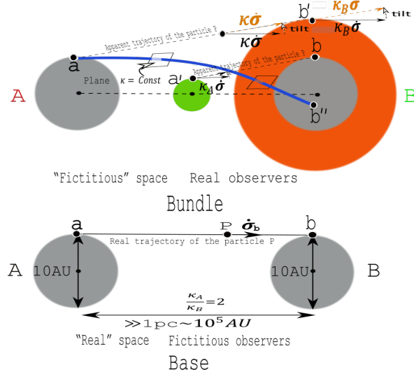
Fig 5 : Two observers A and B separated by a very large distance \gg 1 \text{ pc} . Very close to each of them an universal "atom" of small size \sim 10 \text{ AU} is represented. The dashed straight line \mathbf{ab}' (resp. \mathbf{a}'\mathbf{b} ) is a geodesic of the sheet of the observer A (resp. B) equipped with \kappa_A (resp. \kappa_B ). Let us note that the norm of the vector \dot{\sigma} is a constant in the base, but this norm varies as \frac{1}{\kappa} in the respective sheets of the observers. On the other hand the curve \mathbf{ab} displayed in blue is a geodesic of the bundle equipped of a variable \kappa 9 .
