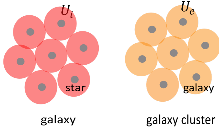
Fig 15 : Stacking of balls covering a galaxy or a galaxy cluster
