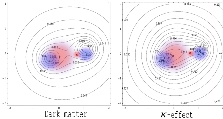
Fig 13 : A comparison between the gravitational lensing diagrams resulting from the application of both dark matter and \kappa -model paradigms in the case of the Bullet Cluster (for the details see [3]).
