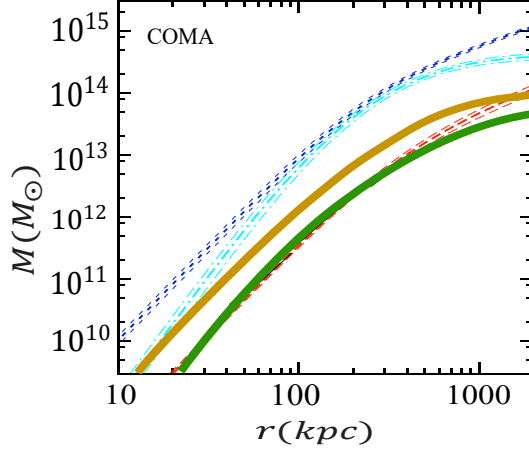
Fig 12 : the short dashed blue curve is the Newtonian dynamic mass; the dashed-dotted cyan curve is the MOND dynamic mass. The dynamic mass for \kappa -model is displayed as the amber curve (dynamic mass with constant temperature T = 8.38 keV) and green curve (assuming a non-isothermal temperature profile). The red long dashed curve is the ICM gas mass derived from X-ray observations (for the details see [3]).
