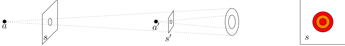
Fig 6.c : Images obtained with kappa-effect, emitter in the central disk see a three time closer, The image of the central disk overlaps the image of the annulus, the overlapping, region is colored in orange
