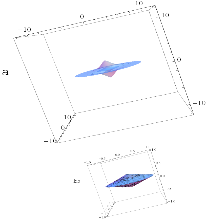
Fig 11 : A side-on galaxy seen by a terrestrial observer (a) as opposed to its compact counterpart living in the base (b). On this illustrative example the terrestrial observer measures the density \rho(r, z) = \exp(-r - (5 + r)|z|) .
