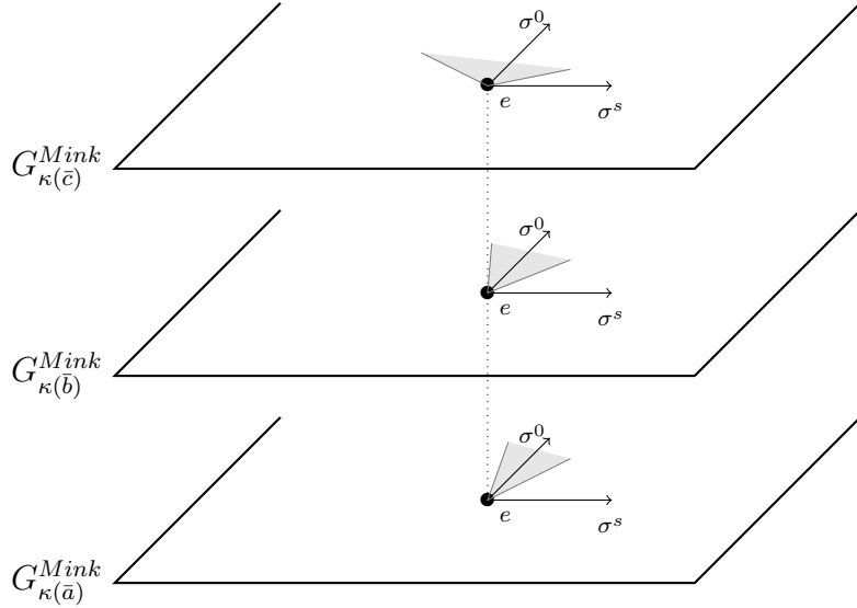
Fig 5 : Deformation of the "future-cone" at e with \kappa(\bar{a}) < \kappa(\bar{b}) < \kappa(\bar{c}) the "space component", \sigma^s , represented in dimension 1
