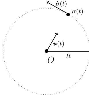
Fig 7 : Circular Newtonian motion
