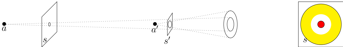
Fig 6.b : Images obtained with kappa-effect, the emitter in the annulus sees the observer a , three time closer. The gap in the image is a consequence of \kappa discontinuity at, the border between the annulus and the central disk
