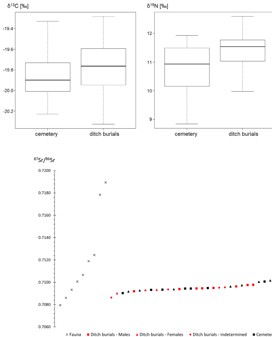
FIGURE 5 Measured ^{87}\text{Sr}/^{86}\text{Sr} ratios from Le Pressoir in Saint-Doulchard (Bourges, France). Grave F206-31, carrier of a distinct plague DNA strain and a dietary outlier, is shown.
