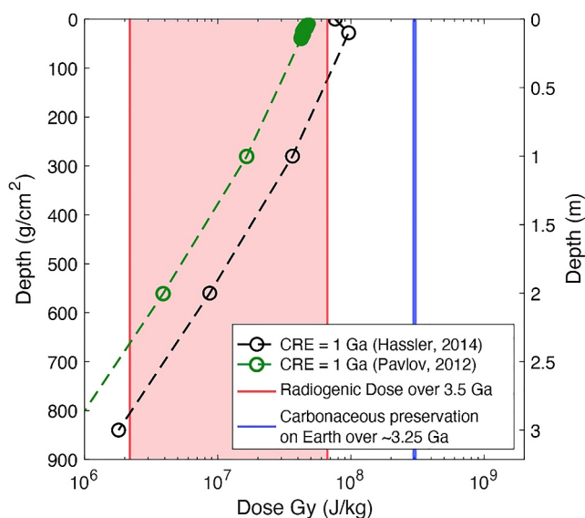
Figure 6. In situ cosmic ray and radiogenic ionizing radiation dose estimates for samples collected from the sedimentary fan front. Depth-dependent radiation doses are shown using dose rate estimates of Hassler et al. (2014) in black and Pavlov et al. (2012) in green, assuming a cosmic ray exposure (CRE) duration of 1 Ga and a constant galactic cosmic ray flux to the surface of Mars for all time since exposure. Time-integrated radiogenic dose from U, Th and K decays over the last 3.5 Ga are shown (red) for K_2O ranging from 0.1 to 3.0 weight percent and assumed K/U and K/Th ratios. For comparison, we estimate the time-integrated radiogenic dose experienced by rocks of the Barberton Greenstone Belt (blue) that preserve carbonaceous lamination (e.g., Hickman-Lewis et al., 2018).
