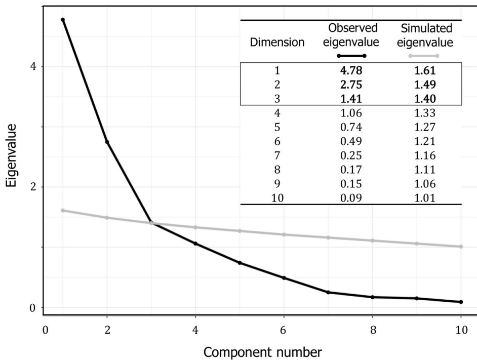
Figure 5. Process for selecting the number of dimensions by comparing the observed and simulated eigenvalues.
