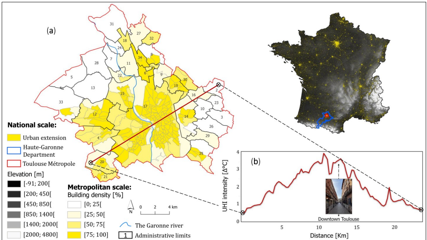
Figure 2. Building density and urban heat island (UHI) intensity in the Toulouse Métropole. (a) Location of the Toulouse Métropole in metropolitan France and urban density within census blocks (IRIS units); (b) UHI intensity along a transect through the city center. Commune names with their numbers are given in Table A1, and the communes and IRIS units covered by the transect are listed in Table A2. Data Sources: IGN-BD ALTI & TOPO (2022); Centre d’Expertise Scientifique “CES Occupation des sols” (OSO); and MApUCE-UHI dataset.
