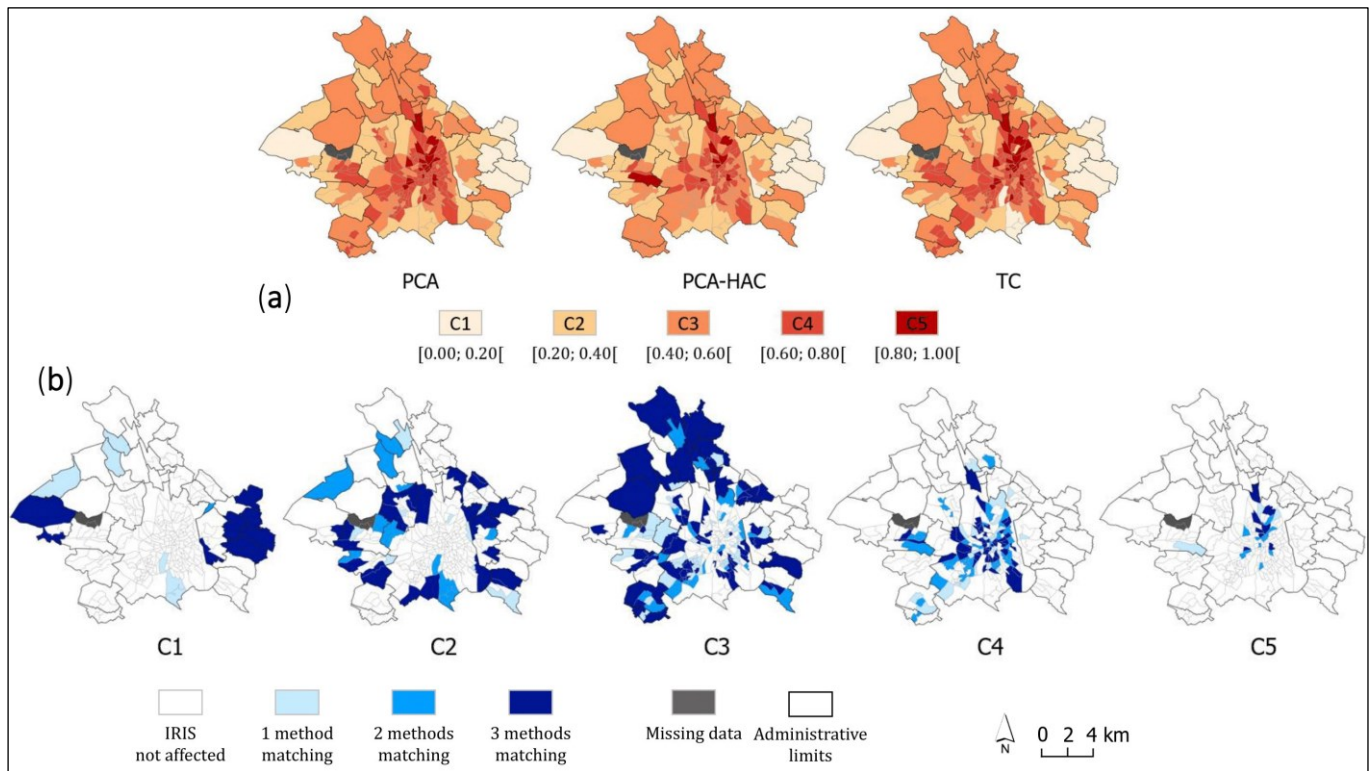
Figure 10. Correspondence of HVI classes according to the method used. (a) Final HVI commonly discretized into equal intervals; (b) number of times the methods classify the same IRIS unit into the same class displayed in panel (a).
