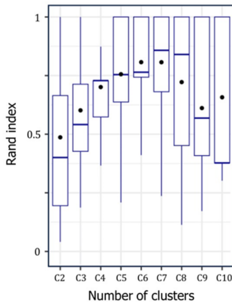
Figure 6. Dispersion of the adjusted Rand index.
