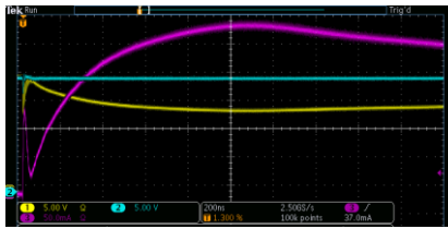
Fig. 6. Waveform of V_{CE} (CH1), V_{IN} (CH2) and I_C (CH3) 200 ns per division V_{IN} = 20V at 120 mW for laser power
