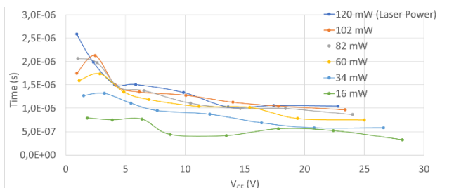
Fig. 9. Switch-on time versus V_{CE} for different laser power from 16 mW to 120 mW
