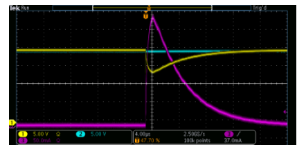
Fig. 7. Waveform of V_{CE} (CH1), V_{IN} (CH2) and I_C (CH3) 4 \mu s per division V_{IN} = 20V at 120 mW for laser power
