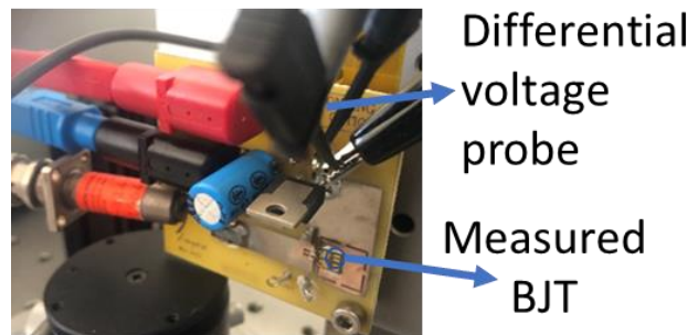
Fig. 4. Photo of the Testbench. Transistor are in the lower right corner
