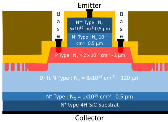
Fig.1. Cross-section of the studied 4H-SiC 10 kV BJT
