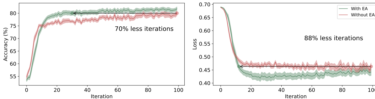
Figure 4: Validation accuracy and loss during training iterations using EEGNet and BCI2014 datasets, with shaded areas depicting the standard deviations over all trained models, one per target subject.
