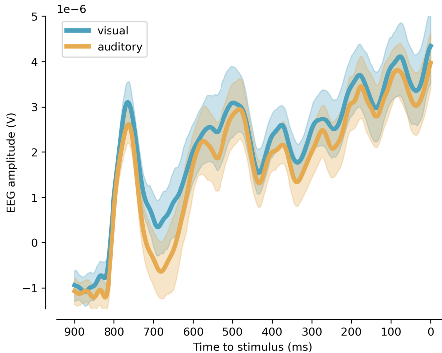
Figure 5: Grand average of anticipatory EEG activity grouped by the type of cue over all participants and channels, with 95% confidence interval over participants. Visual anticipation trials were cued by an eye icon, while auditory anticipation trials were cued by an ear icon.
