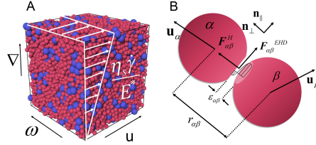
FIG. 1. (A) Configuration of a bidisperse suspension with a volume fraction of \phi = 0.80 with X = 0.10 and r = 1.60 subjected to shear flow with an applied shear rate of \dot{\gamma}\eta_s/E^* in a periodic simulation box. The velocity ( \mathbf{u} ), gradient ( \nabla ), and vorticity ( \omega ) directions are indicated. (B) Schematic showing the pair-wise interaction between particles \alpha and \beta .
