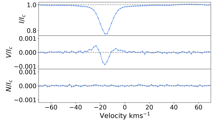
Fig. 1. Least-squares deconvolution profiles for the snapshot observations of HD 63433 with ESPaDOnS. The panels show the Stokes I (top), V (middle) and N (bottom) profiles, obtained from the combination of 4620 atomic spectral lines. We note the presence of a clear Zeeman signature in Stokes V , indicating that the large-scale magnetic field is amenable to characterisation.
