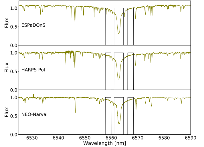
Fig. 2. Normalised fluxes around the H \alpha line for the three instruments used in this study. From the top: ESPaDOnS, HARPSpol, and Neo-Narval. The black rectangles indicate the regions used in the definition of the corresponding activity index. The observations were taken between September 2022 and May 2023.
