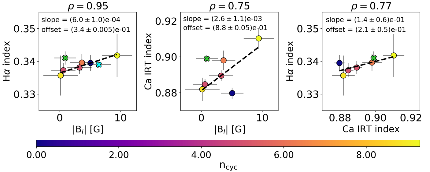
Fig. 4. Correlation plots for the activity proxies computed from the six Neo-Narval observations. From the left: H \alpha vs. |B_l| , Ca II IRT vs. |B_l| , and H \alpha vs. Ca II IRT. Each data point is colour-coded based on the rotational cycle as computed from Eq. (1). Each panel displays the Pearson correlation coefficient ( \rho ) at the top and a linear fit as black dashed line. The green cross indicates the values of the ESPaDOnS snapshot observation, but it was not included in the computation of the Pearson correlation coefficient. We included the first HARPSpol observation in the first panel as a blue cross.
