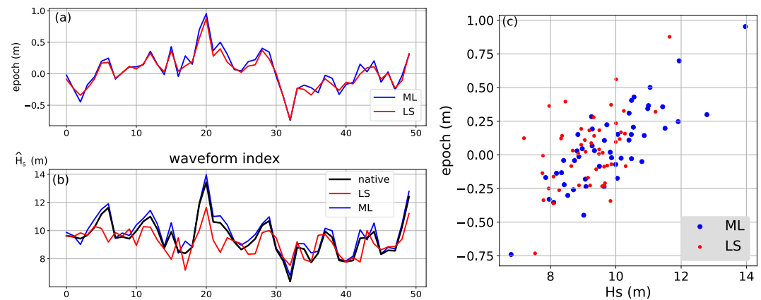
Figure 2. Estimates of the (a) epoch and (b) wave heights for the 50 waveforms of Figure 1b, using two different cost functions: “LS” is a least squares 2-parameter fit to the theoretical waveform given by Equation A17 with a = b = \xi = 0 , \gamma = 1 and “ML” is a maximum likelihood 2-parameter fit to the same theoretical waveform. The “native” data is shown for reference and is the operational method as described in Tourain et al. (2021). The good agreement of the “ML” retracking with the “native” data requires to ignore the first range gates using k_{\min} \approx 80 , or adapting k_{\min} such that S(k_{\min}) > r_{\min} \max(S) , with r_{\min} \approx 0.06 .
