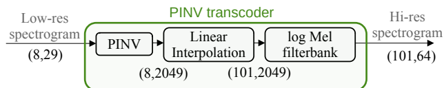
FIG. 1. PINV transcoder architecture, to recover a 1s sample fine spectrogram from a 1s sample coarse spectrogram
