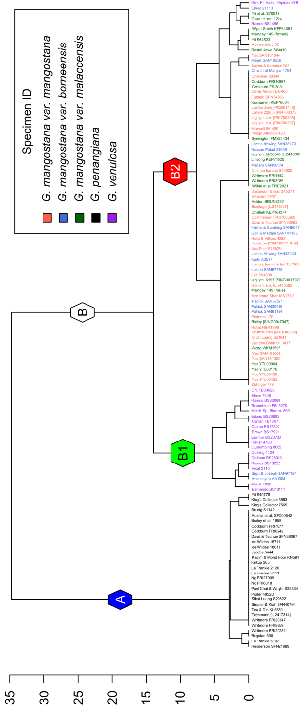
Figure 3. Ascendant hierarchical classification dendrograms for the vegetative key characters specimen subset.
