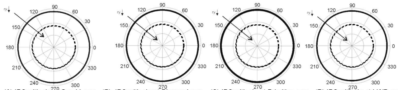
(A) IPC with sheet Gyroid core (B) IPC with sheet Diamond core (C) IPC with sheet Primitive core (D) IPC with sheet I-WP core FIGURE 14. DIRECTIONAL SHEAR AND LONGITUDINAL PHASE WAVE PROPAGATION VELOCITY (KM/S) IN UHPC-STEEL IPCS WITH SHEET TPMS CORES.
