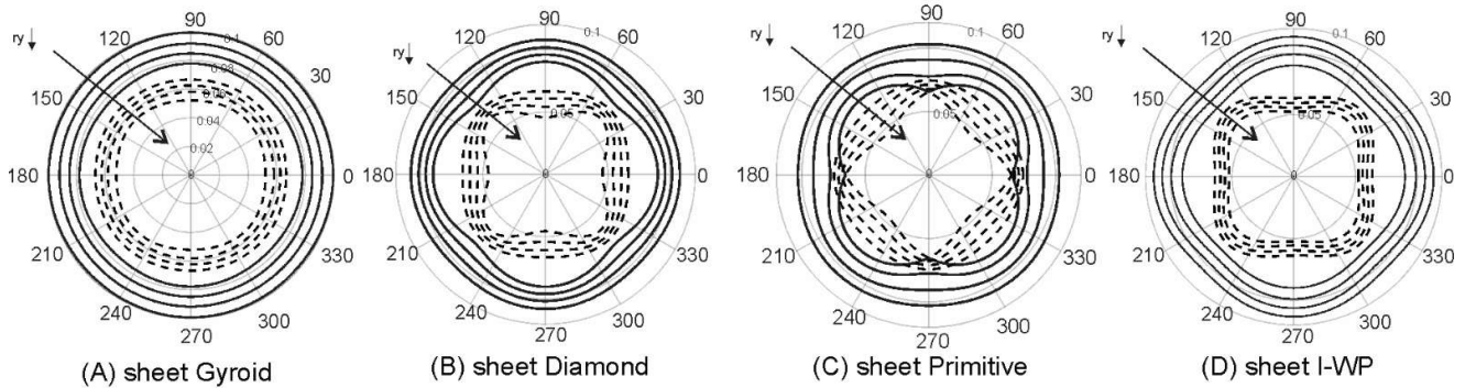
(A) sheet Gyroid (B) sheet Diamond (C) sheet Primitive (D) sheet I-WP FIGURE 13. DIRECTIONAL SHEAR AND LONGITUDINAL LONG-FREQUENCY IMPACT PHASE WAVE VELOCITY (KM/S) PROPAGATING IN UHPC-BASED SHEET TPMS BEAMS.
