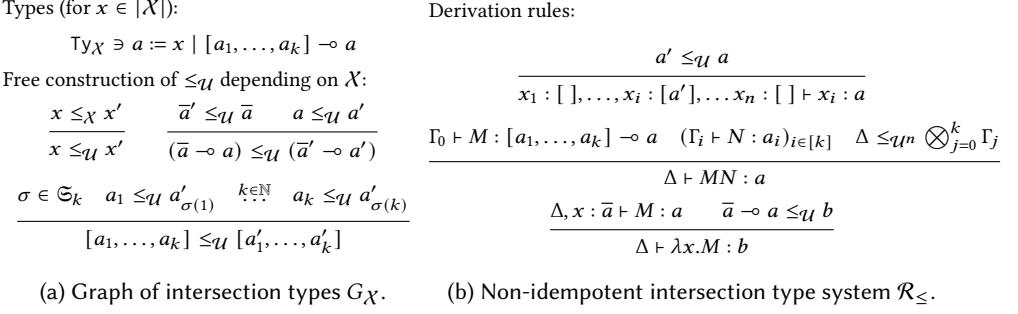
Fig. 6. Type theoretic presentation of a relational graph model living in Polr.
