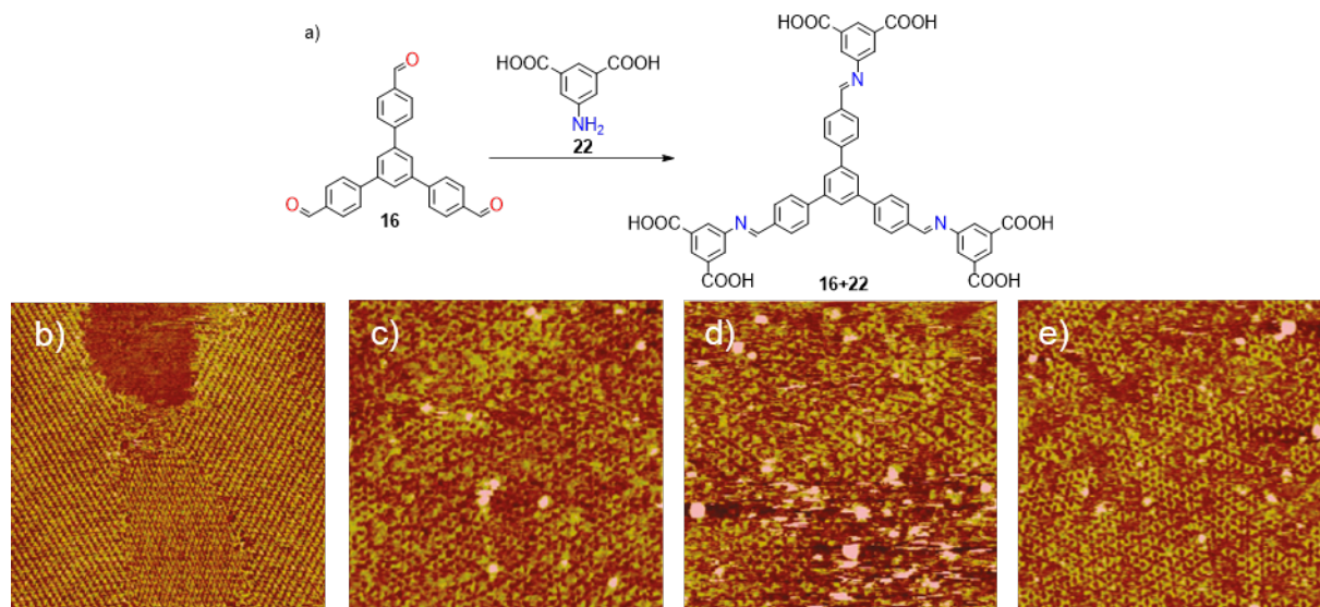
Figure 5. Schematic representation of condensation reaction of aldehyde 16 with amine 22 (a) and series of STM sequence images of a 70.0 nm x 70.0 nm region illustrating the structural transformation: (b) lamellar structure of aldehyde 16 ; (c) irregular structure formed upon addition of amine 22 on pre-existing aldehyde 16 layer; (d) the open network after 12h and (e) 24 h. Imaging conditions: V_{\text{bias}} = 935.3 mV and I_t = 223.3 pA). Reproduced from Ref., [74] with permission of American Chemical Society.
