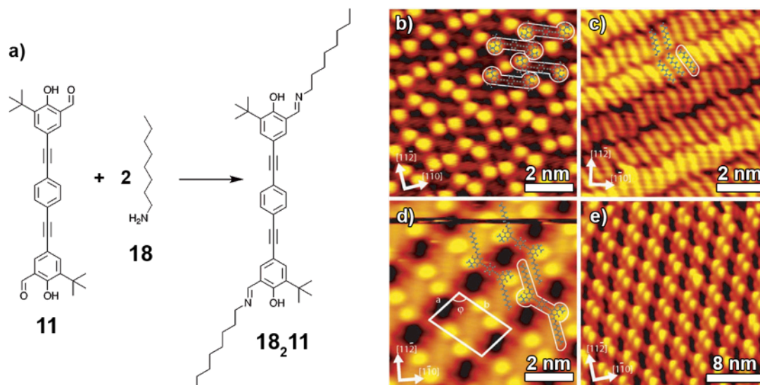
Figure 3. (a) Schematic representation of condensation reaction of aldehyde 11 with amine 18 on a Au(111) surface. STM images of (b) self-assembled island formed by the dialdehyde 11 ; (c) lamellar structure formed by 18 ; (d) self-assembled structure formed by the bis-imine 18 2 11 prepared in situ at room temperature. The unit cell of the structure is indicated; (e) large ordered domain formed by the bis-imine prepared in situ . Imaging conditions: (b) I_t = -0.77 nA, V_t = -1.0 V; (c) I_t = 0.41 nA, V_t = +2.0 V; (d) I_t = 0.27 nA, V_t = +1.9 V; (e) I_t = -0.42 nA, V_t = -2.2 V, bar size 4 nm. Reproduced from Ref., [73] with permissions of Wiley.
