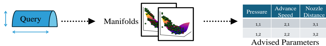
Fig. 11. Inverse model based on the manifolds predicted using the Machine Learning direct model to advice optimal sets of process parameters
