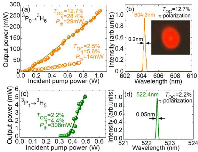
Fig. 4. Pr:LiYF 4 surface channel waveguide lasers: (a,b) Orange laser, the ^3P_0 \rightarrow ^3H_6 transition; (c,d) Green laser, the ^3P_1 \rightarrow ^3H_5 transition: (a,c) input-output dependences, \eta – slope efficiency, P_{th} – laser threshold; (b,d) spectra of laser emission, \pi -polarization. Inset – photograph of the orange laser beam in the far-field.
