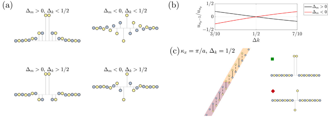
Fig. 4. Localized mode shapes and dimer chain for \Delta_k = 1/2 . (a) Mode shapes in a decoupled state at \kappa_x = \pi/a for obtained for \Delta_m = +1/5 > 0 (left column), \Delta_m = -1/5 < 0 (right column), \Delta_k = 1/5 < 1/2 (upper row), and \Delta_k = 4/5 > 1/2 (lower row), decay of modes from the interface. (b) Ratio of u_{n_p-1}/u_{n_p} , \Delta_k transverse the value 1/2 has a transition through zero. (c) Decoupling of masses for \Delta_k = 1/2 at the wavenumber \kappa_x = \pi/a showing perfectly isolated bound modes (marked under the green square and red diamond) in the band gap.
