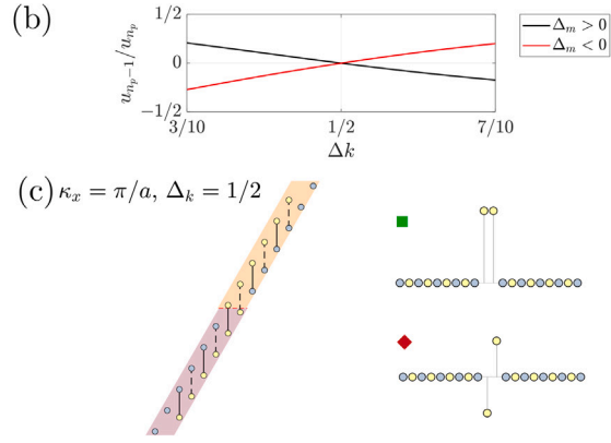
Fig. 4. Localized mode shapes and dimer chain for \Delta_k = 1/2 . (a) Mode shapes in a decoupled state at \kappa_x = \pi/a for obtained for \Delta_m = +1/5 > 0 (left column), \Delta_m = -1/5 < 0 (right column), \Delta_k = 1/5 < 1/2 (upper row), and \Delta_k = 4/5 > 1/2 (lower row), decay of modes from the interface. (b) Ratio of u_{n_p-1}/u_{n_p} , \Delta_k transverse the value 1/2 has a transition through zero. (c) Decoupling of masses for \Delta_k = 1/2 at the wavenumber \kappa_x = \pi/a showing perfectly isolated bound modes (marked under the green square and red diamond) in the band gap.
