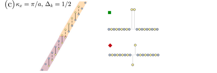
Fig. 4. Localized mode shapes and dimer chain for \Delta_k = 1/2 . (a) Mode shapes in a decoupled at \kappa_x = \pi/a for obtained for \Delta_m = +1/5 > 0 (left column), \Delta_m = -1/5 < 0 (right column), \Delta_k = 1/5 < 1/2 (upper row), and \Delta_k = 4/5 > 1/2 (lower row), decay of modes from the interface. (b) Ratio of u_{n_p-1}/u_{n_p} , \Delta_k transveres the value 1/2 has a transition through zero. (c) Decoupling of masses for \Delta_k = 1/2 at the wavenumber \kappa_x = \pi/a showing perfectly isolated bound modes (marked under the green square and red diamond) in the band gap.
