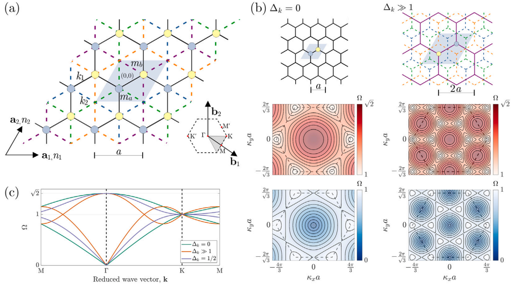
Fig. 1. Discrete elastic lattice and associated dispersion diagrams. (a) Hexagonal lattice described by the lattice vectors \{\mathbf{a}_1, \mathbf{a}_2\} , with unit cells with indices (n_1, n_2) and pairs of masses (m_a, m_b) connected to the nearest (third nearest) neighboring masses through springs of stiffness k_1 ( k_2 ) denoted by continuous black (dashed colored) lines. The light blue parallelogram denotes the reference unit cell (0,0) . The reciprocal lattice (basis vectors \{\mathbf{b}_1, \mathbf{b}_2\} ) and high-symmetry points ( \Gamma, K, K', M, M' ) are also shown. (b) Hexagonal lattices (top panels) and dispersion surfaces (middle and bottom panels) for \Delta_k = 0 (left panels) and \Delta_k \gg 1 (right panels). The unit cells in each case are highlighted in light blue. The lattice for the case \Delta_k \gg 1 corresponds to 4 unconnected copies (represented by different colors) of the lattice for the \Delta_k = 0 case, with double spacing. One of these 4 lattice is represented in continuous lines (purple) for the sake of clarity. (c) Dispersion curves for \Delta_k = 0, \Delta_k = 1/2 , and \Delta_k \gg 1 .
