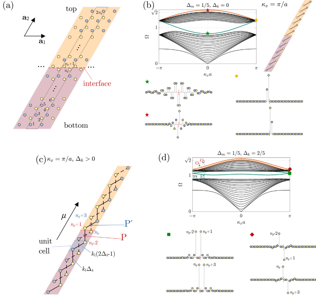
Fig. 3. Dispersion diagrams and localized modes in a finite strip. (a) Lattice with periodicity in the a_1 -direction and a finite length in the a_2 -direction, presenting an interface between the top ( \Delta_{m,t} , in orange) and bottom ( \Delta_{m,b} = -\Delta_{m,t} , in purple) regions. (b) Dispersion curves for \Delta_m = 1/5 , \Delta_k = 0 , with branches having even (green) and odd (red) symmetries enveloping the bulk bands, whose wave modes are shown at \kappa_x = 0 (green and red stars, respectively). These modes converge to a set of bound modes in the continuum, showing the localized motion of pairs of masses (yellow circle) due to decoupled consecutive unit cells (top right panel). (c) Decoupled pairs of dimer chains at \kappa_x = \pi/a with symmetry at the point P (P') for the chain marked with continuous (dashed) lines. (d) Dispersion curves computed for \Delta_m = 1/5 , \Delta_k = 2/5 . The even (odd) modes indicated as E_1/E_2 ( O_1/O_2 ) (O 1 /O 2 ) and highlighted in green (red) merge into bound modes marked by the green square (red diamond) at \kappa_x = \pi/a , who display even (odd) symmetry about the P (P') point, relative to masses n_p - 2/n_p + 1 ( n_p/n_p + 3 ).
