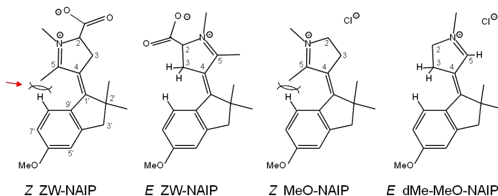
Figure 7. Schemes of the ground state structures of various NAIP compounds. In the Z isomer of ZW-NAIP, steric hindrance between the methyl group carried by C_5 and the hydrogen carried by C_8 induces a 13^\circ torsion of the C_{1'}=C_4 bond (see SI of [29]). In the E -ZW-NAIP, the methyl substitute of C_5 can fit between both methyl groups carried by C_{2'} , but residual stress induces significant pyramidalization of C_{1'} and C_4 (among other deformations) and produces a non-planar structure too. In the case of Z -MeO-NAIP, the C_{1'}=C_4 bond is twisted by 11^\circ in the ground state [27]. Instead in the dMe-MeO-NAIP, where C_5 carries a H atom instead of the methyl group, the E isomer is planar.
