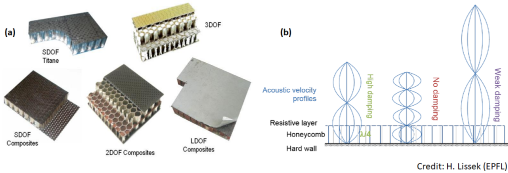
Figure 10 – Single and multi-degree-of-freedom liners (a), whose functioning is based upon the quarter-wavelength principle (b).
