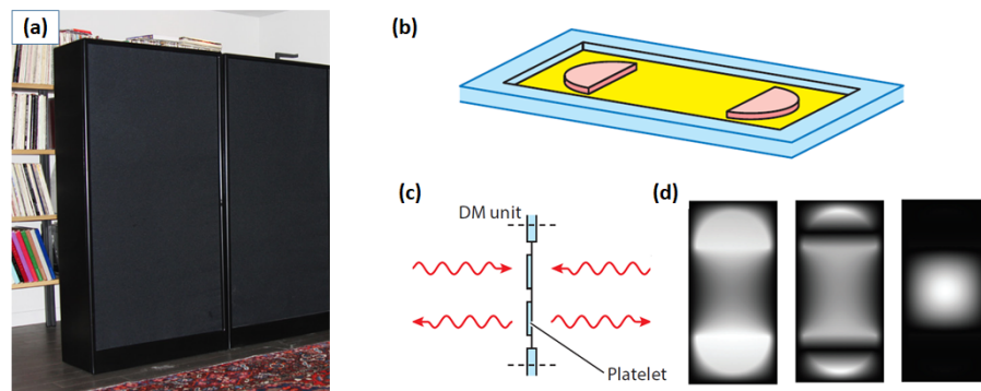
Figure 9 – Membrane bass-trap for room acoustics (a) from www.andymacdoor.com ; sketches of the decorated membrane (DM) (b), (c) with the additional masses (platelets), providing the multimodal behaviour (d), from [11].
