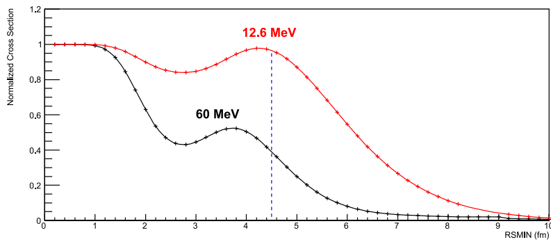
Fig. 35. The normalized total cross section is shown as a function of the RSMIN parameter. This is calculated with the FRESKO code for the ^{18}\text{F}(d,n)^{19}\text{Ne}^* transfer reaction to the 3/2^+ state at E_x = 6289 keV in ^{19}\text{Ne} at two beam energies, 60 MeV and 12.6 MeV. The RSMIN parameter is used to set the overlap form factor to zero inside the interval r < \text{RSMIN} in the ^{19}\text{Ne} = ^{18}\text{F} + p system [163,174]. The radius of the ^{19}\text{Ne} nucleus is shown with the vertical dashed line. The effect of the RSMIN parameter becomes noticeable (significant reduction of the cross section) at \text{RSMIN} = 1.7 fm at an incident energy of 60 MeV, and at 5.2 fm at 12.6 MeV. This shows that the transfer reaction occurs mostly at the surface of the nucleus ( r \approx 5 fm) at 12.6 MeV, and much deeper inside ( r \approx 2 fm) at 60 MeV.
