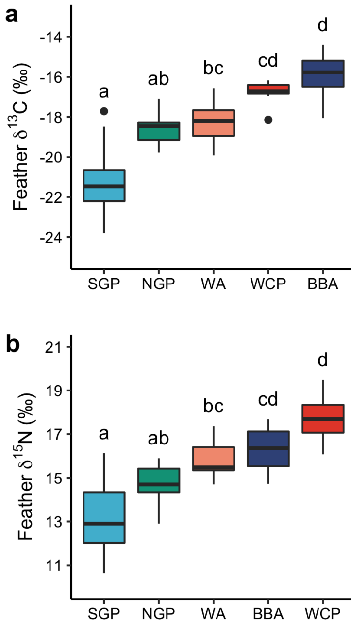
Fig. 3. Boxplots of (a) carbon ( \delta^{13}\text{C} ) and (b) nitrogen ( \delta^{15}\text{N} ) stable isotope values (‰) in body feathers of albatrosses and large petrels sampled at Bird Island, South Georgia. Species abbreviations are: BBA = black-browed albatross Thalassarche melanophris ; NGP = northern giant petrel Macronectes halli ; SGP = southern giant petrel M. giganteus ; WA = wandering albatross Diomedea exulans ; WCP = white-chinned petrel Procellaria aequinoctialis . Samples were collected from southern giant petrels in the 2011/12 breeding season and from all other species in 2014/15. Species sharing superscript letters are not significantly different according to post-hoc Dunn's tests. Boxplots show medians (horizontal lines), interquartile range (IQR; boxes), the lowest and highest values within 1.5 x IQR (whiskers) and outliers (black points).
