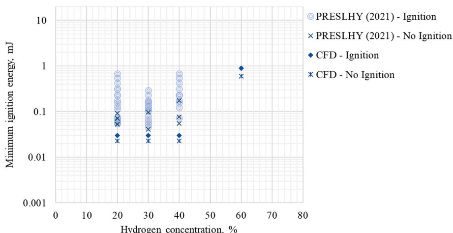
Fig. 7. MIE in hydrogen-air mixture at T_0 = 173 K: CFD simulations against PRESLHY experiments (2021) [25].
