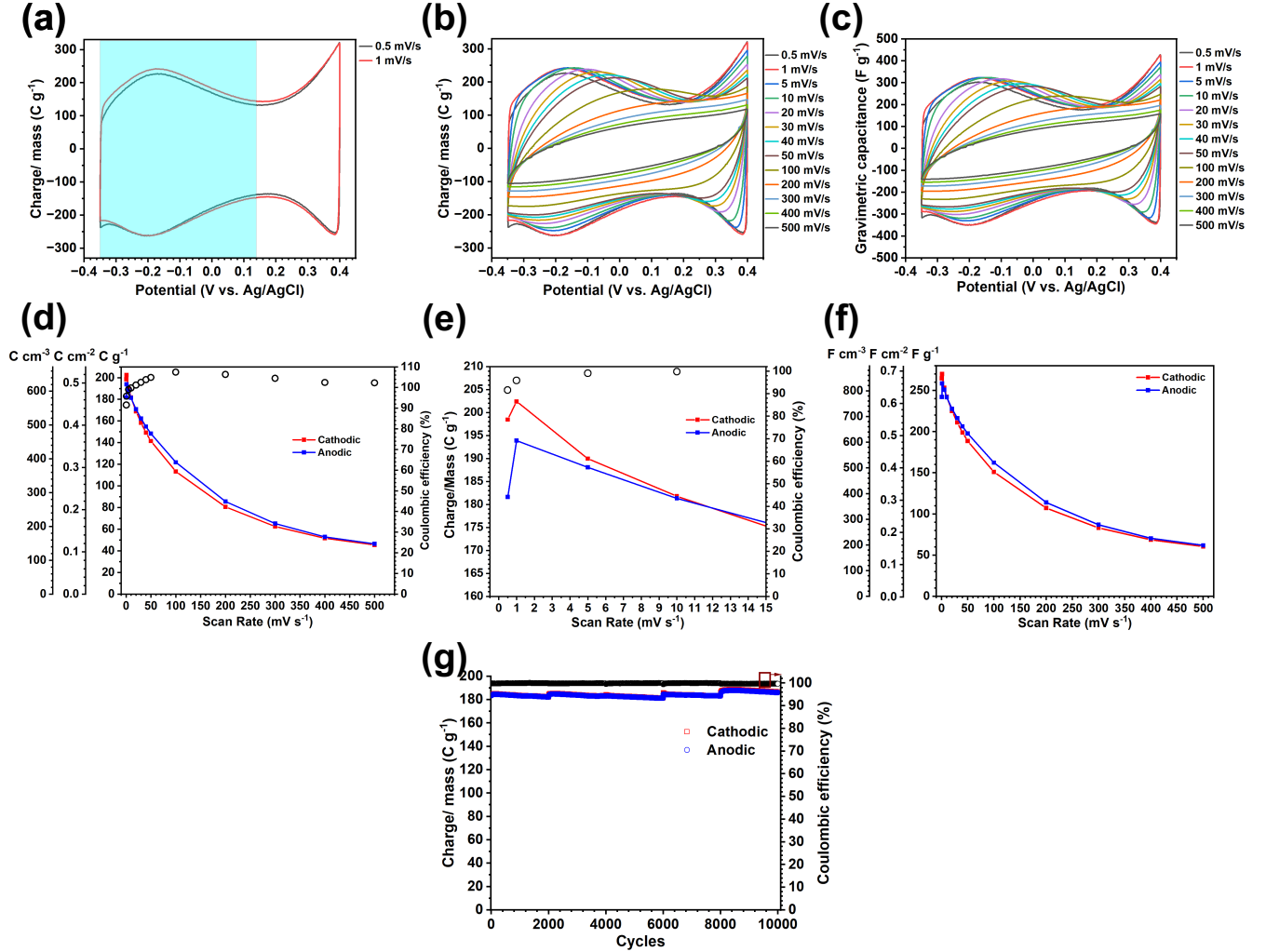
Figure 5: Cyclic voltammetry tests of V_4C_3T_x film electrodes in a half-cell set up using Ag/AgCl as reference electrode and 3 M H_2SO_4 electrolyte. CVs (second cycle) at (a) 0.5 and 1 mV s -1 and (b)-(c) 0.5 to 500 mV s -1 , (d-e) corresponding charge storage and (f) capacitance vs. scan rate curves - notice that (e) is the inset of (d) -, (g) charge storage vs. cycle number curves calculated from CVs run at 10 mV s -1 . The charge storage is presented in (a)-(b) C g -1 and (c) F g -1 . In (a) the potential region affected by ion starvation, and where charge storage processes involve mass transport control (as further explained in section 3.4) is colored.
