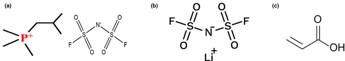
Figure 1. a) P 11114 FSI ionic liquid. b) LiFSI salt. c) Acrylic acid monomer.
