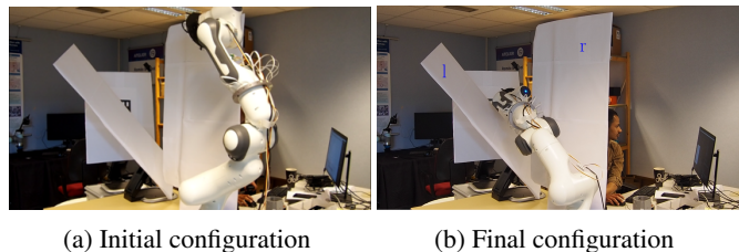
Fig. 4: Experimental setup for Case 1 consisting of Panda robot, two obstacles, and 4-point target.
