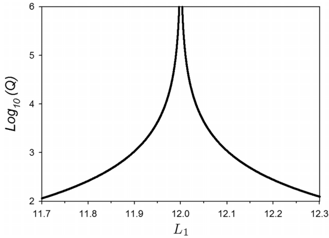
FIG. 9. Variation of the logarithm of the quality factor Q of the peaks reported in Fig. 8 as a function of the stub length L_1 . One can notice that the quality factor of the peak depends on the value of L_1 and as predicted diverges when L_1 = 12 nm.
