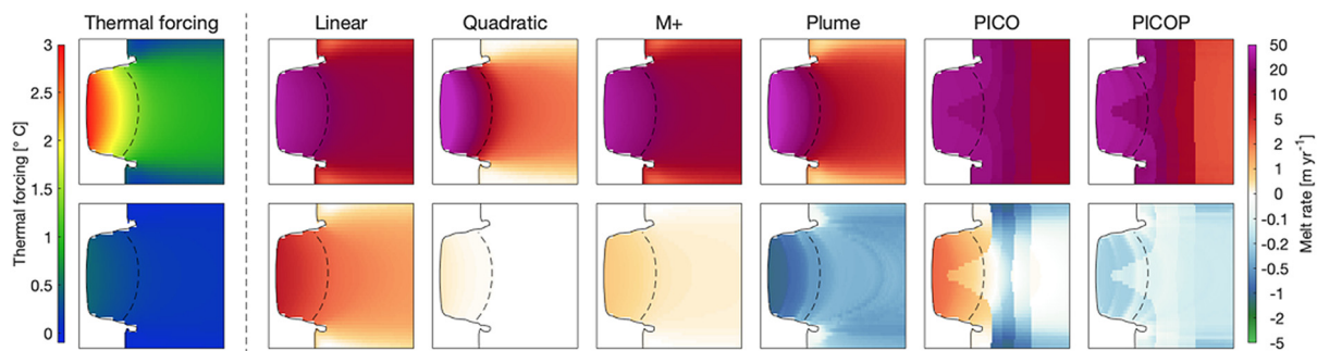
Figure 7. First column: thermal forcing at the shelf base, for the WARM (upper row) and COLD (lower row) ocean profiles in the MISMIP+ steady-state geometry. Other columns: sub-shelf melt rates produced by the six different melt parameterisations. The 300 m shelf draft contour and the grounding line are indicated by the dashed and solid black lines, respectively.
