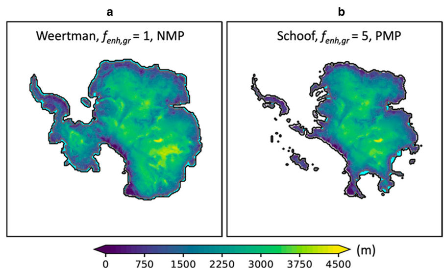
Figure 9. Ice thickness at the end of the 500-year ABUMIP ABUM experiment, using (a) Weertman sliding, f_{\text{enh,gr}} = 1 , NMP, and (b) Schoof sliding, f_{\text{enh,gr}} = 5 , PMP, both at 32 km resolution. Cyan areas indicate remnants of ice shelves. These are respectively the least and most responsive simulations of the ensemble.
