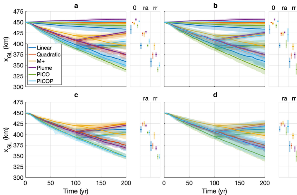
Figure 8. Grounding-line position over time in the MISOMIP1 experiments. (a) IceOcean1 experiments (fixed ice front). (b) IceOcean2 experiments (fixed ice front + threshold-thickness calving). (c) IceOcean1 experiments relative to the IceOcean0 control. (d) IceOcean2 experiments relative to the IceOcean0 control. Bars on the right-hand side of the panels indicate range of grounding-line positions per melt model at the end of each experiment (with 0 = cold ocean, rr = warm ocean and ra = 100 years warm followed by 100 years cold). Each shaded area represents the ensemble of six simulations for a single melt parameterisation, e.g. the green shaded area indicates the range of values resulting from the three sliding laws and two resolutions, when using the PICO melt parameterisation.
