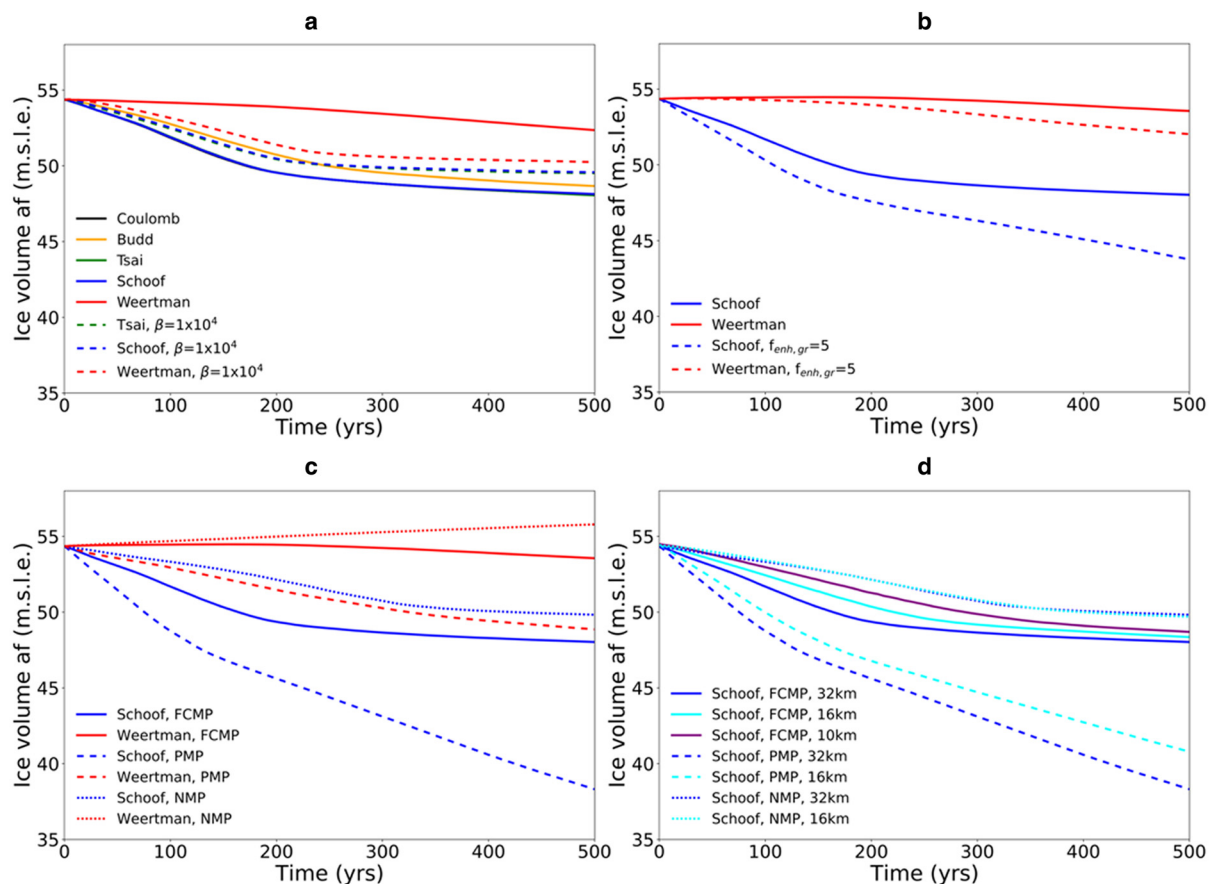
Figure 10. (a) Evolution over time of ice volume above flotation in the ABUMIP ABUM experiment using (a) different sliding laws and basal roughness (32 km resolution, FCMP, f_{\text{enh,gr}}=1 ) (solid green, black and blue lines overlap, only blue is visible), (b) different flow enhancement factors (32 km resolution, FCMP), (c) different sub-grid melt schemes (32 km resolution, f_{\text{enh,gr}}=1 ), and (d) different resolutions ( f_{\text{enh,gr}}=1 ).
