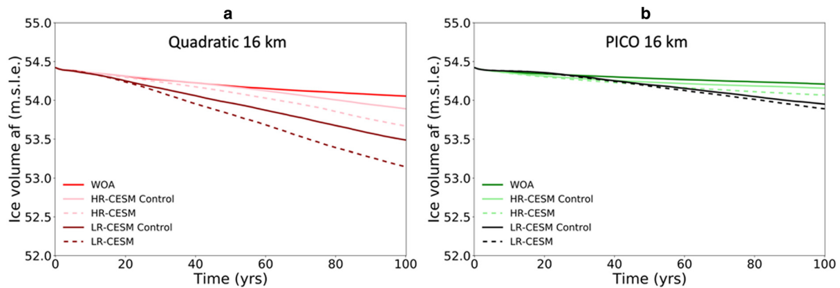
Figure 14. (a) Evolution over time of ice volume above flotation in the experiments using ocean forcing from WOA, and low-resolution (LR) and high-resolution (HR) CESM (control and perturbed) simulations, with quadratic sub-shelf melt and (b) PICO, at 16 km resolution.
