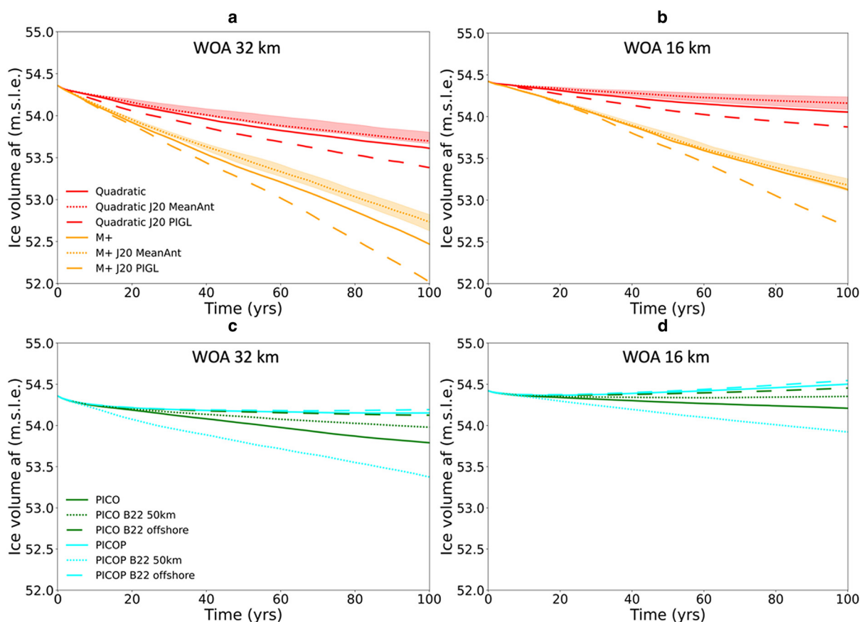
Figure 12. (a) Evolution over time of ice volume above flotation (af) in the experiments using ocean forcing from World Ocean Atlas (WOA) data at 32 km resolution and (b) at 16 km resolution, with quadratic and M+ sub-shelf melt parameterisations using MISOMIP tuning, and using parameter settings obtained from Jourdain and others (2020) [J20]. The shading envelopes the range yielded by the 5th to the 95th percentile values of the MeanAnt tuning. The dotted and dashed lines represent the median values of the MeanAnt and PIGL tunings respectively. (c–d) Same for the PICO and PICOP sub-shelf melt parameterisations using MISOMIP tuning, and using parameter settings obtained from Burgard and others (2022) [B22]. The parameter settings for these experiments are listed in Table 6.
