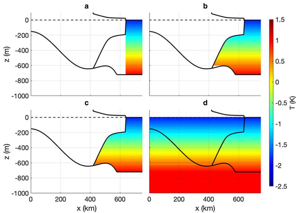
Figure 3. Demonstrating the cavity extrapolation protocol from Jourdain and others (2020) in the MISIMIP+ geometry. (a) Ocean temperature data are provided only on the open ocean. (b) The data are extrapolated horizontally into the shelf cavity. The bottom part of the cavity is blocked by the sill, and is therefore not treated by the horizontal extrapolation step. (c) The data are extrapolated vertically, filling in the bottom part of the cavity. (d) The data are extrapolated both horizontally and vertically into the ice and bedrock, providing values for all parts of the domain that might at any point in time become submerged by the changing ice and bed geometry.
