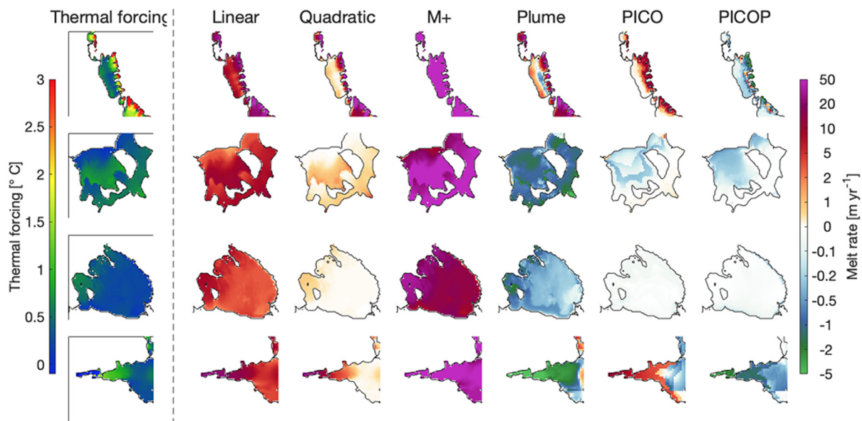
Figure 13. Thermal forcing (leftmost column), and sub-shelf melt rates underneath the ice shelves at the start of the experiments at 16 km resolution using ocean forcing from World Ocean Atlas (WOA) data. Different sub-shelf melt parameterisations are applied, using parameter values as calibrated in the MISOMIP1 experiment (Table 6). For the forcing and each parameterisation, the rows show (top to bottom) the Amundsen Sea embayment, the Filchner–Ronne embayment, the Ross embayment and the Amery embayment.
