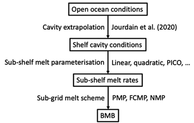
Figure 2. The relation between open ocean conditions and ice-sheet basal mass balance can be separated into the following three conceptual steps: (1) cavity extrapolation, (2) sub-shelf melt parameterisation and (3) sub-grid melt scheme.
