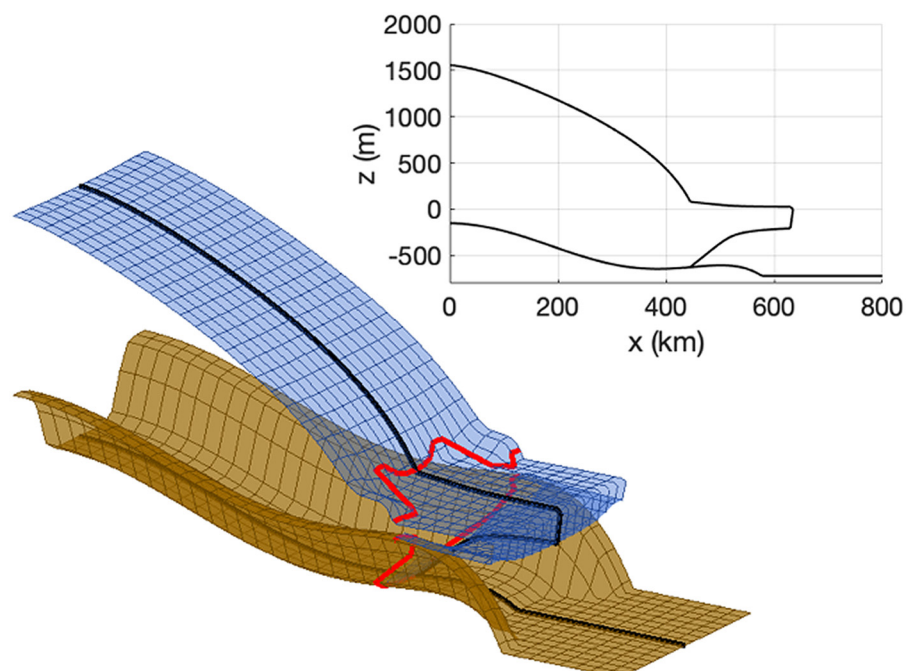
Figure 4. The MISIMIP+ idealised geometry. The grounding line and its projection on the ice surface are shown in red; a cross-section along y=0 is shown in the top-right panel. z=0 is equal to sea level, which is kept constant in time.
