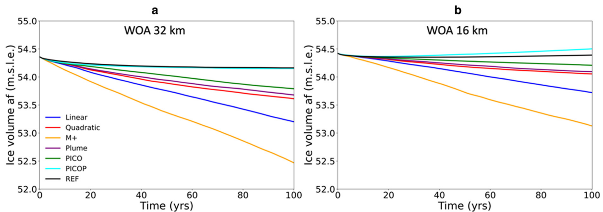
Figure 11. (a) Evolution over time of ice volume above flotation (af) in the experiments using ocean forcing from World Ocean Atlas (WOA) data at 32 km resolution and (b) at 16 km resolution, with different sub-shelf melt parameterisations using parameters tuned following the MISOMIP protocol, and with fixed ice-shelf geometry for reference (REF; first 100 years of the ABUMIP ABUC experiment).
