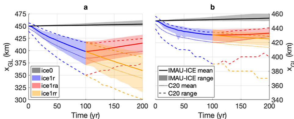
Figure 5. Grounding-line position over time in the MISMIP+ experiments, compared to the model intercomparison results by Cornford and others (2020). For IMAU-ICE, the ensemble mean is indicated by a solid line, and the range by the shaded areas. For Cornford and others (2020), the ensemble mean is indicated by a dotted line, and the range by dashed lines. (a) ice0, ice1rr and ice1ra. (b) ice0, ice2rr and ice2ra. Mind the differing y-axis scales.
