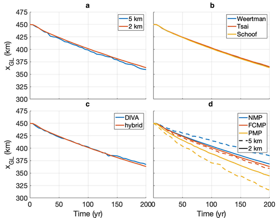
Figure 6. Grounding-line position over time in the MISMIP+ ice1rr experiment, separated by the choice of (a) resolution, (b) sliding law, (c) stress balance approximation and (d) sub-grid melt scheme. The default choices are 2 km resolution, Schoof2005, DIVA and FCMP. This means that e.g. the blue line in panel A has all of these, except for the resolution, which is 5 km.
