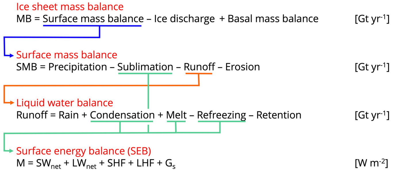
Fig 2. Definitions of ice sheet mass balance (MB), surface mass balance (SMB) and liquid water balance, all ice-sheet integrated mass fluxes expressed in gigatonnes per year (Gt yr -1 ). ‘Basal mass balance’ refers to ablation at the ice-bedrock interface. ‘Erosion’ refers to removal of snow by wind, ‘Retention’ to the irreducible water content of porous snow. Note that the definition of SMB used here includes processes in the firn layer, and is formally referred to as ‘climatic mass balance’ [64]. Surface Energy Balance (SEB) is defined locally and expressed in watts per square metre (W m -2 ). SEB symbols are explained in the main text. Adapted from [65].
