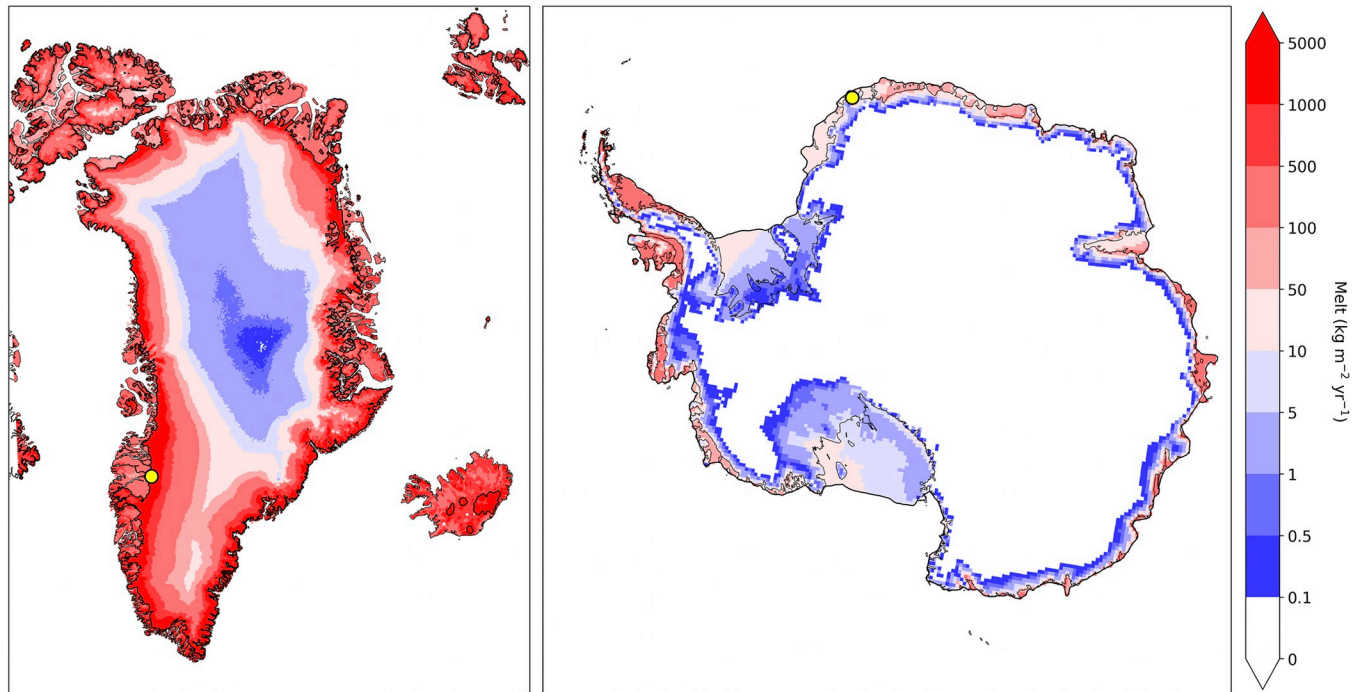
Fig 4. Modelled average (1991–2020) annual melt on the GrIS (left, 0,05 latitudinal degree or \sim 5.5 km resolution) and the AIS (right, 0,25 latitudinal degree or \sim 27 km resolution) from the polar regional climate model RACMO2.3p2. Continuous black lines indicate grounded ice sheet margin or coastlines. Yellow dots indicate locations of AWS S5 (Greenland) and Neumayer base (Antarctica). Note the nonlinear melt scale. Made with Natural Earth (Public Domain, https://www.naturalearthdata.com/about/terms-of-use/ ).
